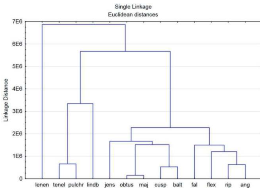
Figure 3. Tree diagram of 13 species by 23 climatic factors.
