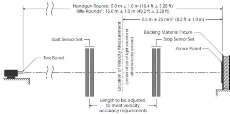
Figure 8. Shooting arrangement [4].
