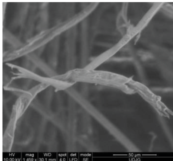
Figure 12. Fibrillation of fibers (front view, code 2F-1).
