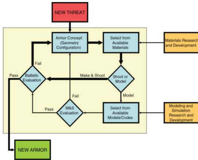
Figure 3. Flow chart of new or redesigned armor [10].
