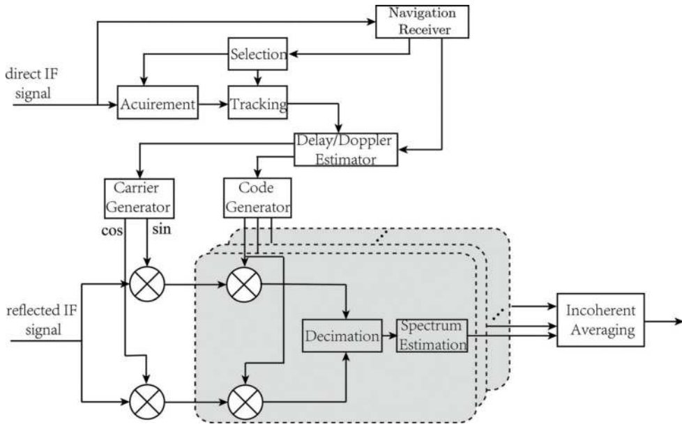
Figure 9. Block diagram of parallel in Doppler domain.
