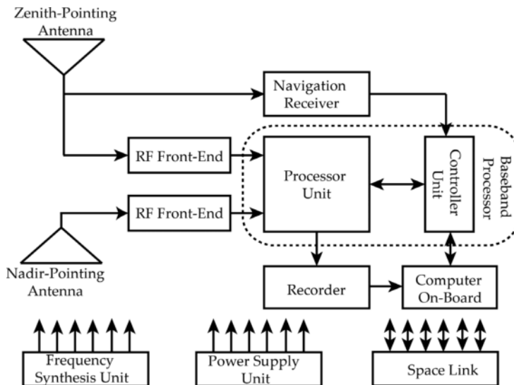
Figure 6. Architecture of Spaceborne GNSS-R receiver.
