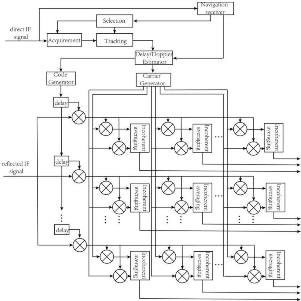
Figure 7. Block diagram of serial correlation method.
