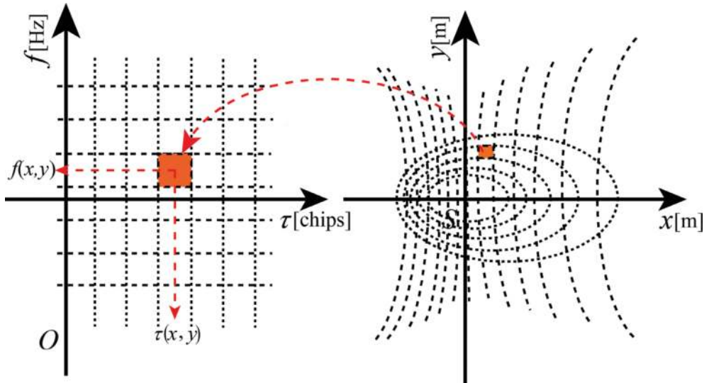
Figure 5. Mapping from space to the delay-Doppler domain.
