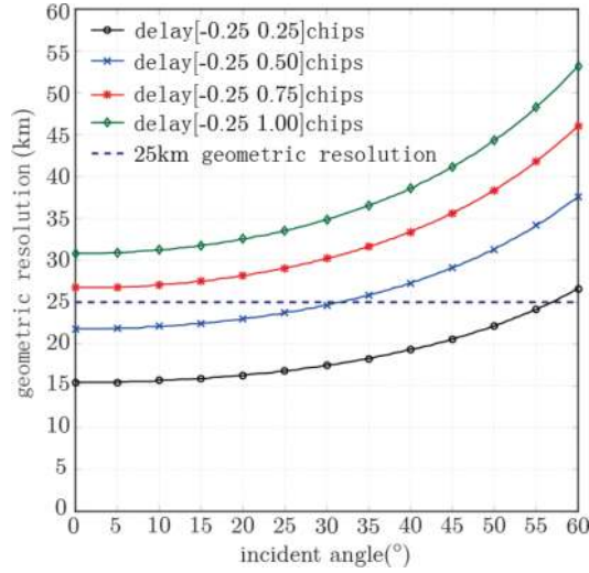
Figure 14. Relationship between geometric resolution and incident angle.
