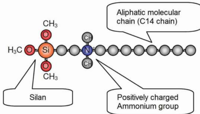
Figure 2. Schematic chemical structure of tested antimicrobial agent.
