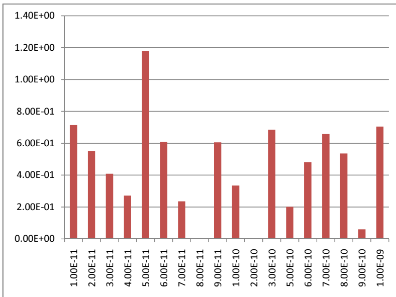
Figure 13. Relative error (%) versus photocurrent (A).
