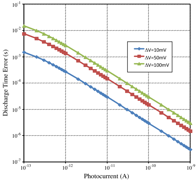
Figure 3. Discharge time error.
