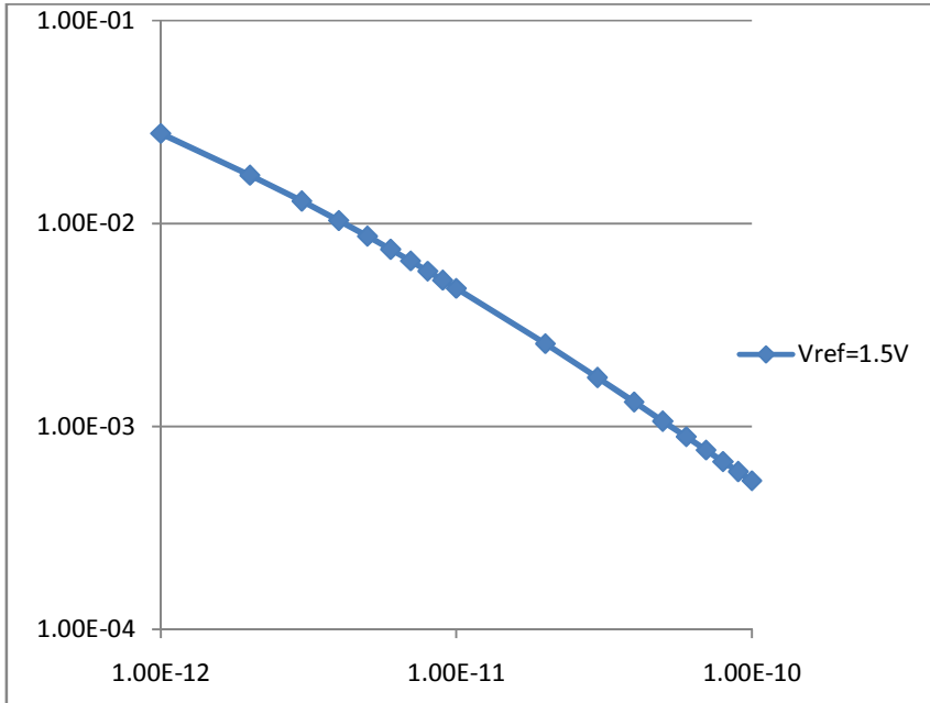
Figure 8. Discharge time (s) versus photocurrent (A).
