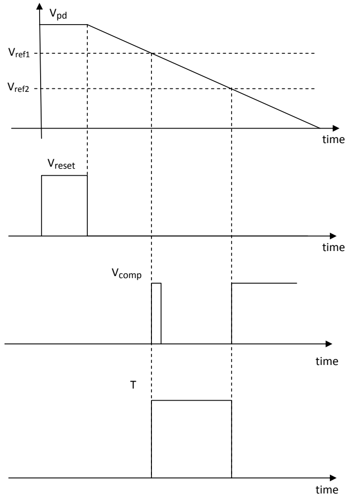
Figure 15. Electronic circuit main waveforms.
