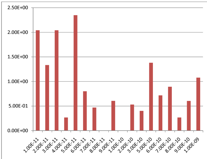
Figure 11. Relative error (%) versus photocurrent (A).
