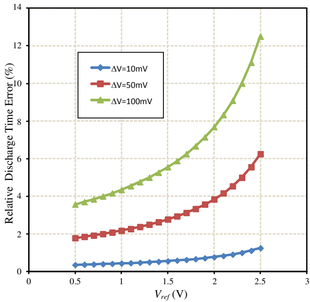
Figure 4. Relative discharge time error.
