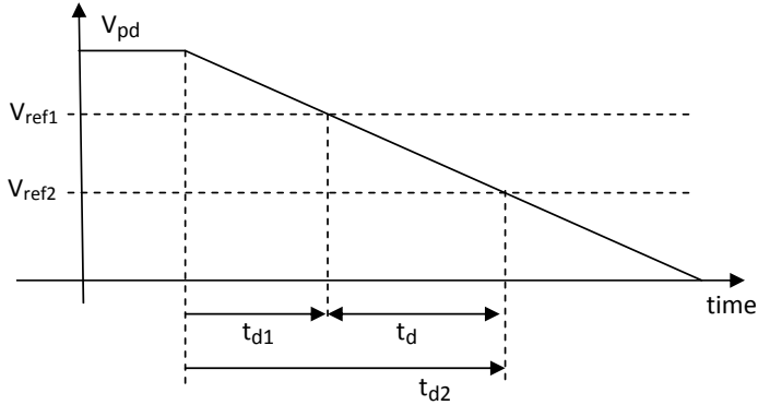
Figure 5. New readout method main waveforms.
