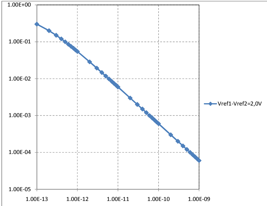
Figure 6. Discharge time (s) versus photocurrent (A).
