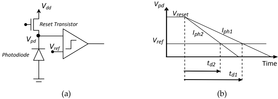
Figure 1. (a) Time-domain CMOS pixel; (b) main waveforms.
