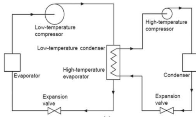
Figure 7. Systematic diagram of the multistate system.
