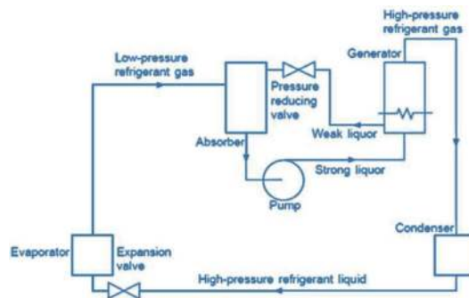
Figure 3. Vapor absorption refrigeration systems.
