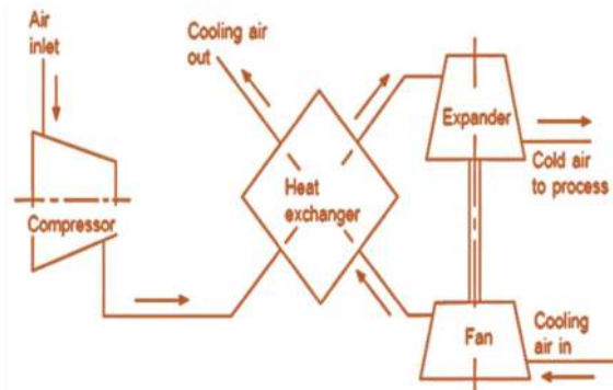
Figure 5. Air or gas expansion refrigeration systems.
