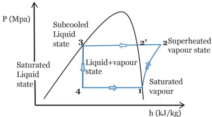
Figure 1. P-h diagram of a vapor compression cycle.
