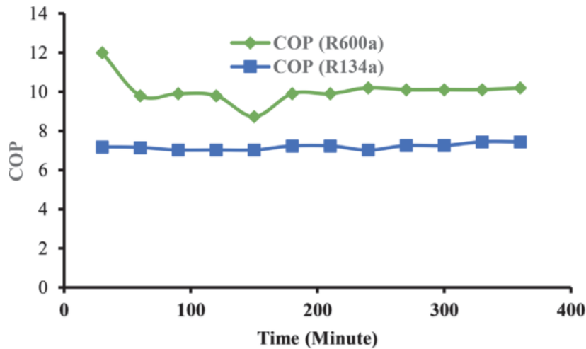
Figure 10. Coefficient of performance with time.
