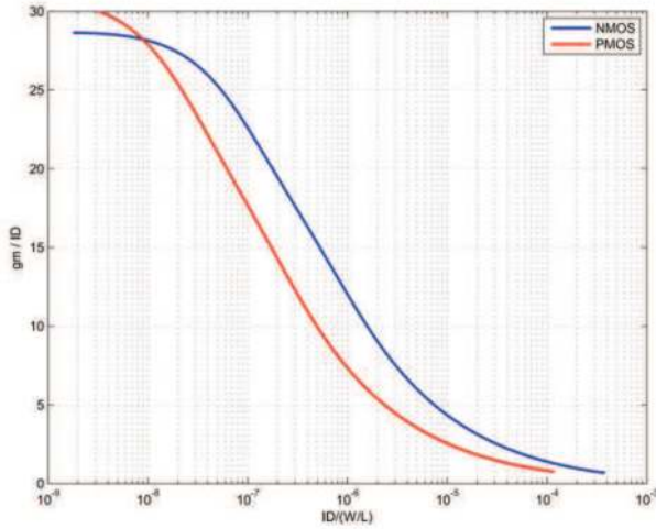
Fig. 3. gm/I_D \times I_D/(W/L) curves for 0.35\mu m CMOS technology.
