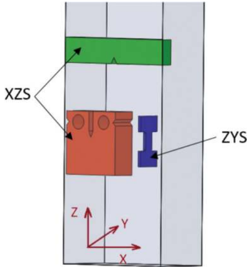
Figure 11. Orientation and designation of the specimens for the material Ti6Al4V produced SLM AM technology (Z = building direction).
