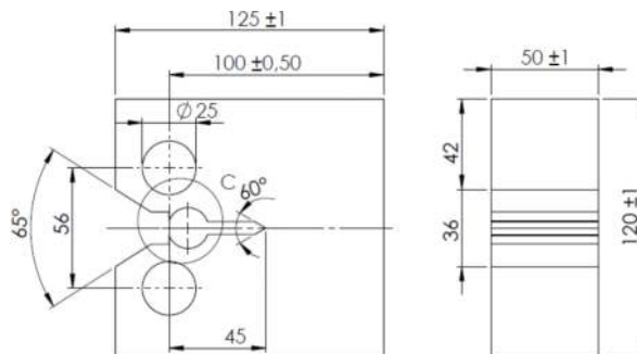
Figure 10. 2 T-CT specimen geometry.
