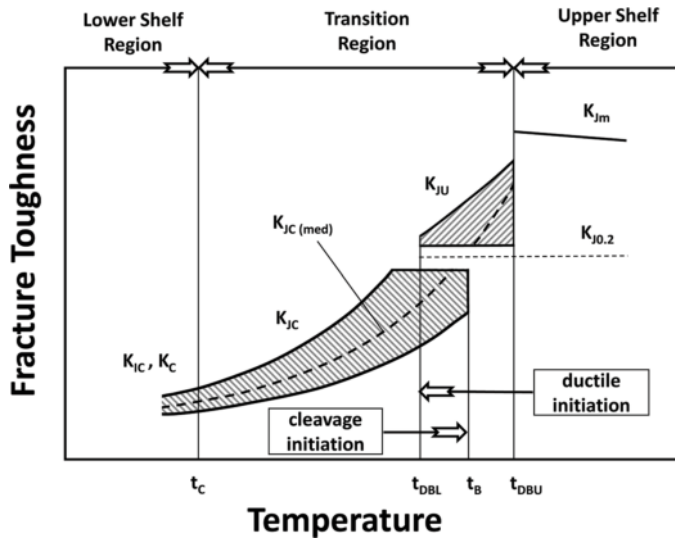
Figure 1. Schematic representation of fracture toughness-temperature dependence.
