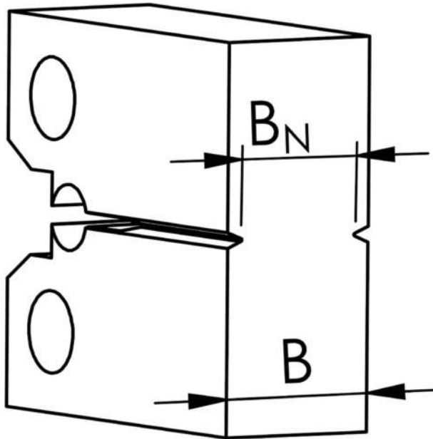
Figure 4. Side grooves in a fracture mechanics test specimen.
