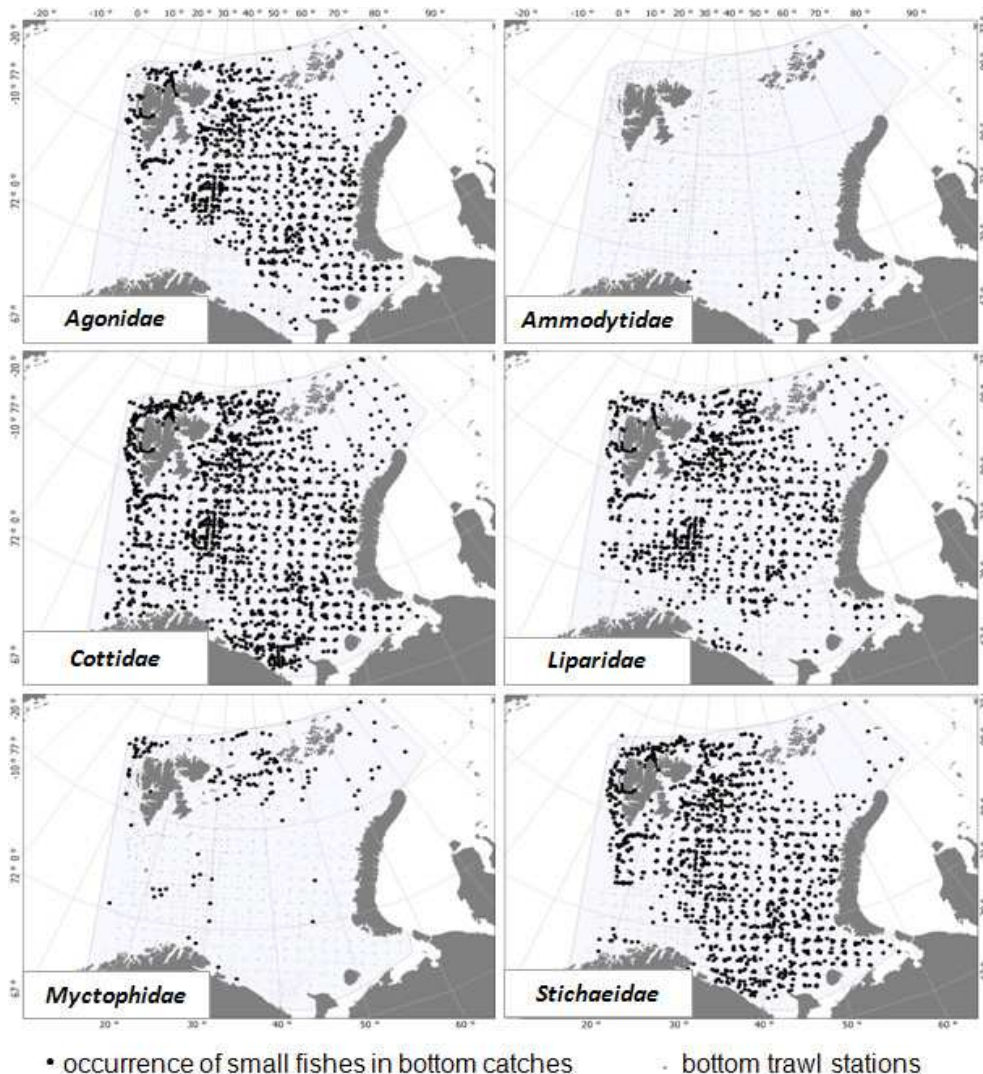
Fig. 3. Spatial distribution of demersal Agonidae , Ammodytidae , Cottidae , Liparidae , Myctophidae and Stichaeidae in the Barents Sea during 2004-2009. Occurrence of small fishes in bottom catches is shown by black circles, while grey and small circles showed bottom trawl stations.
