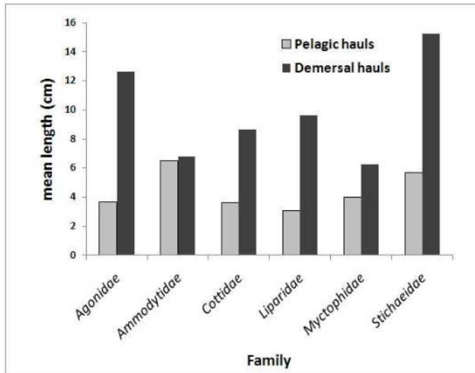
Fig. 4. Mean length of small species from pelagic and bottom trawl catches.
