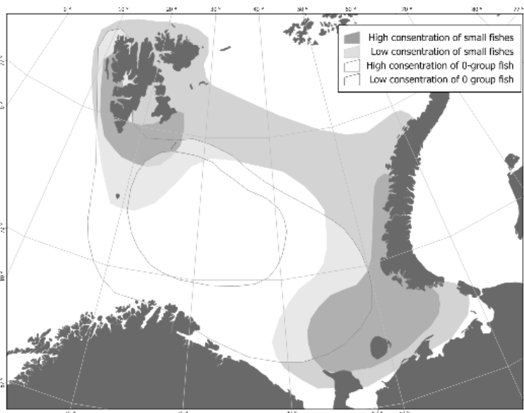
Fig. 5. Distribution of 0-group (cod, haddock, herring and capelin) and small fishes. The distribution of 0-group fish is modified from Eriksen and Prozorkevich 2011 and Eriksen et al. (2011).
