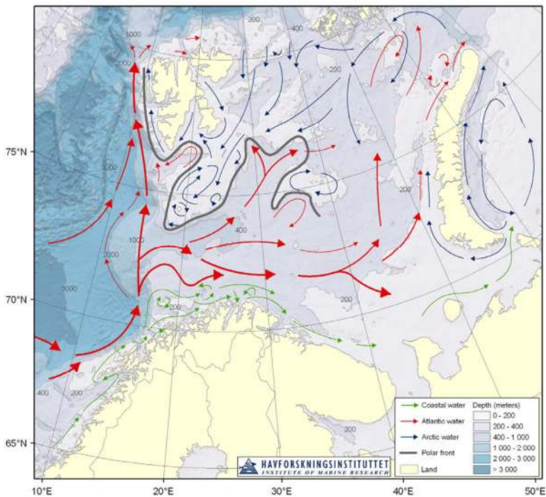
Fig. 1. Overview of the Barents Sea geography and current system.
