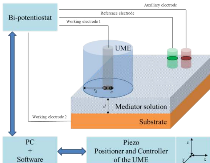
Figure 1. Scheme of SECM instrumentation. The basic parts are as follows: a piezo positioner and a controller of the UME, a bi-potentiostat and PC (with measuring software). The UME scans the substrate surface due to moving the UME by the piezo positioner. The system can work in a three- or four-electrode setup (with connected second working electrode).
