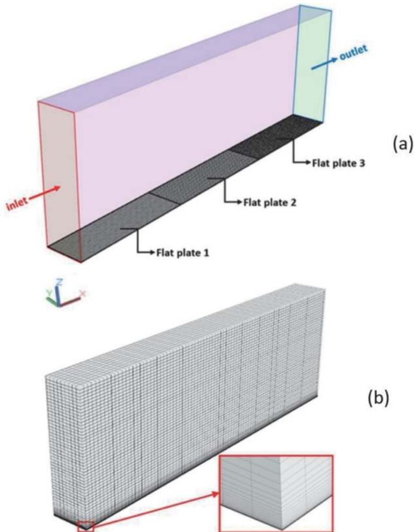
Figure 1. The flow domain used in the simulations with three plate segments at the bottom boundary (a), and the hexahedron mesh with an exponential cell height gradation near the wall bottom boundary (b).
