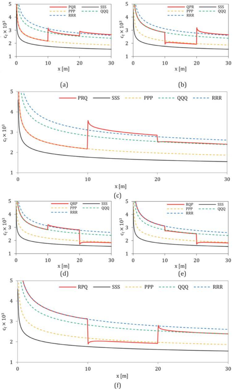
Figure 4. The distribution of local skin friction coefficient c_f along the plate length for the inhomogeneous PQR (a), PRQ (c), QPR (b), QRP (d), RPQ (f), and RQP (e) cases compared with the homogeneous SSS, PPP, QQQ, and RRR cases.
