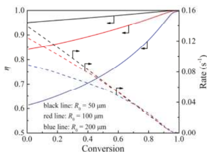
Figure 13. Calculated results of effectiveness factor and reaction rate against particle conversion under different particle sizes at 800\text{ }^{\circ}\text{C} .
