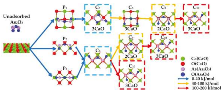
Figure 6. Overall adsorption paths of \text{As}_2\text{O}_3 on CaO.
