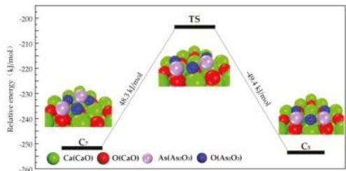
Figure 4. Transformation path of Category III.
