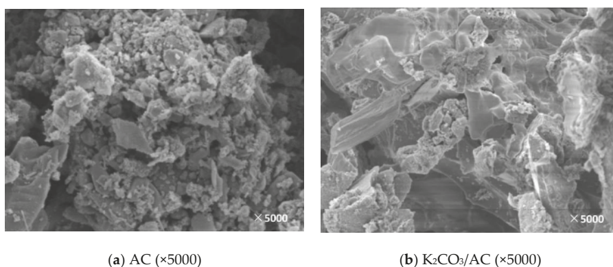
Figure 5. SEM image before and after AC loading. (a): The SEM image of AC; (b): The SEM image of \text{K}_2\text{CO}_3/\text{AC} .
