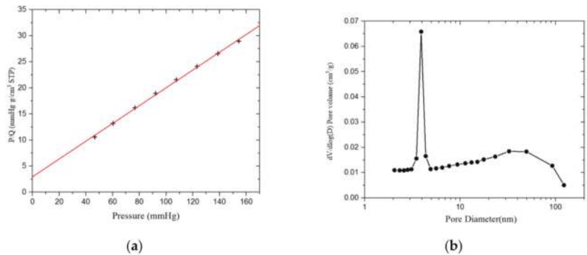
Figure A3. Nitrogen adsorption of sample 1 measured by an ASAP 2420 instrument (Micromeritics Instrument Corp., Norcross, GA, USA). (a) Langmuir surface area plot; (b) BJH desorption dV/d\log(D) pore volume.
