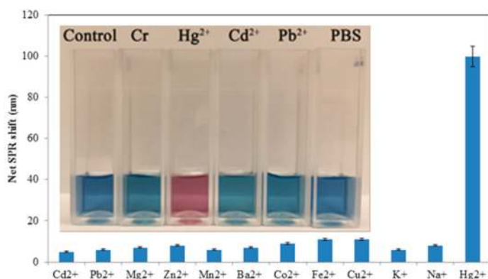
Figure 9. Effect of various metal ions ( 5 \mu\text{M} ) dissolved in 5 \text{ mM} phosphate buffered saline \text{pH } 7.2 on the net SPR shift, showing high reactivity with only \text{Hg}^{2+} . Inset: photograph of AgNP solutions, showing color change with \text{Hg}^{2+} and lack of significant response to phosphate-buffered saline (PBS), deionized water (Control), and the other ions \text{Cd}^{2+} , \text{Pb}^{2+} and \text{CrO}_4^{2-} (labelled “Cr”) at 10 \mu\text{M} .
