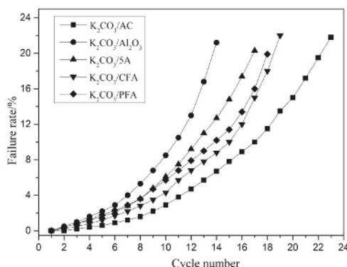
Figure 14. Cyclic experimental results of different adsorbents.
