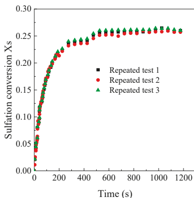
Figure 5. The repeated test results (Samcheok limestone, 26.3\ \mu\text{m} , 850\ ^\circ\text{C} , 1000 ppm).
