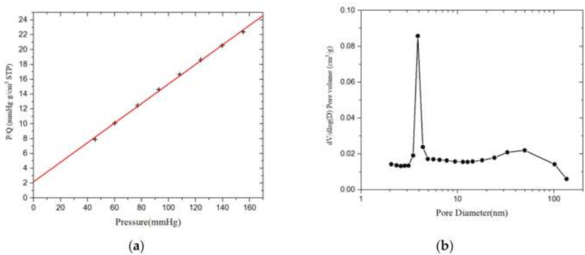
Figure A4. Nitrogen adsorption of sample 2 measured by an ASAP 2420 instrument (Micromeritics). (a) Langmuir surface area plot. (b) BJH desorption dV/d\log(D) pore volume.
