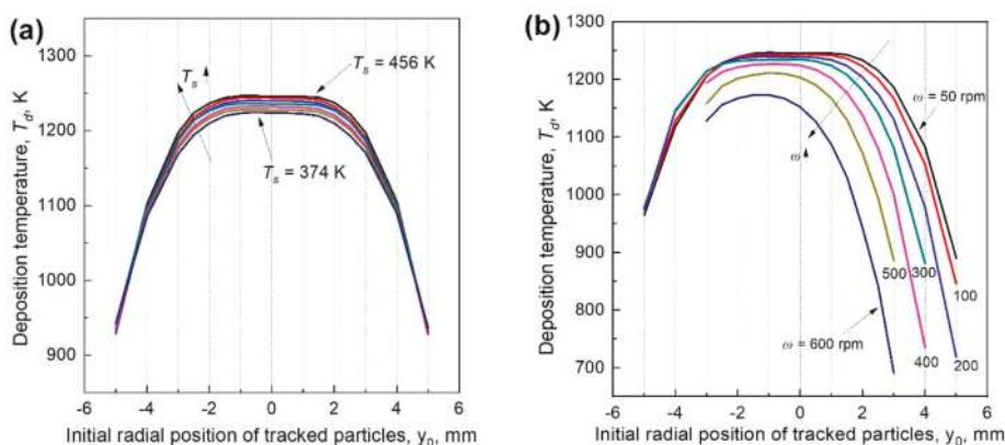
Figure 11. Deposition temperature of the tracked particles when the stagnation surface is (a) in stationary and (b) rotates at different speeds.
