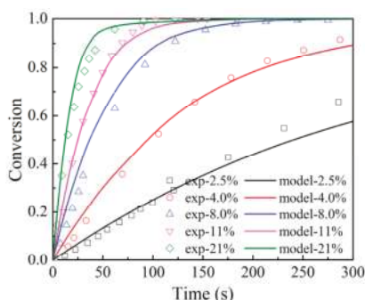
Figure 4. Effects of \text{O}_2 volume percentage (vol%) on conversion at 900 °C. ( [\text{O}_2] = 2.5\text{--}21 vol%, \text{N}_2 as equilibrium gas. Dots: experimental data [42]; lines: model results.)
