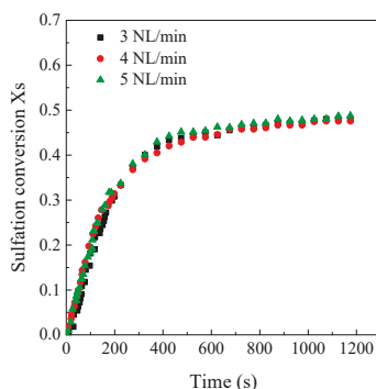
Figure 4. The sulfation conversion under different gas flow rate (Shengzhou limestone, 3.5\ \mu\text{m} , 850\ ^\circ\text{C} , 500 ppm).
