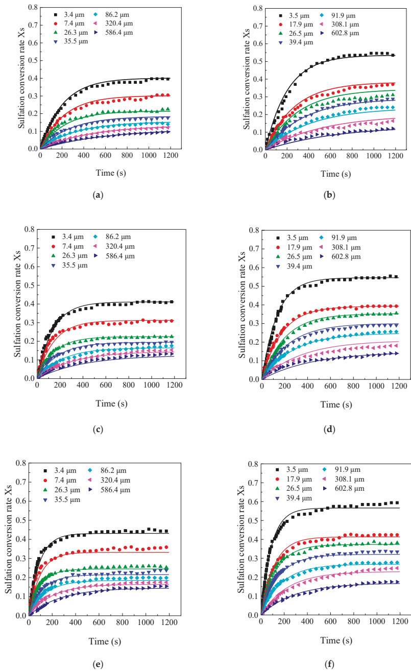
Figure 9. The sulfation conversion at different \text{SO}_2 concentrations under 850^\circ\text{C} : (a) Samcheok, 250 ppm; (b) Shengzhou, 250 ppm; (c) Samcheok, 500 ppm; (d) Shengzhou, 500 ppm; (e) Samcheok, 1000 ppm; (f) Shengzhou, 1000 ppm.
