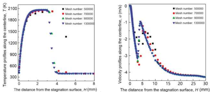
Figure 3. Mesh independence test: (a) Temperature profiles along the centerline of the flame at different mesh number; (b) velocity profiles along the centerline of the flame at different mesh number.
