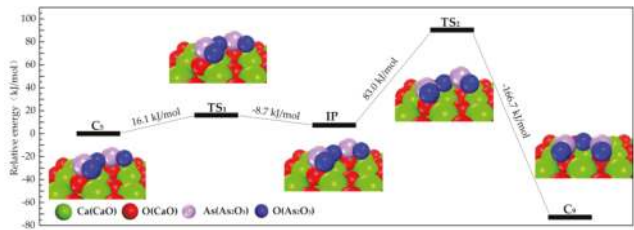
Figure 3. Transformation path of Category II.
