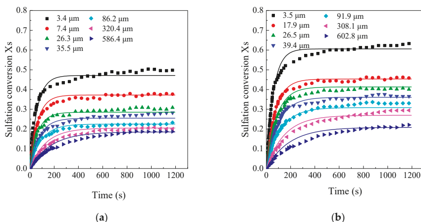
Figure 8. Effects of limestone particle size on the CaO sulfation reactivity (the large capacity TGA, 850 ^{\circ}\text{C} , 2000 ppm): (a) Samcheok; (b) Shengzhou.
