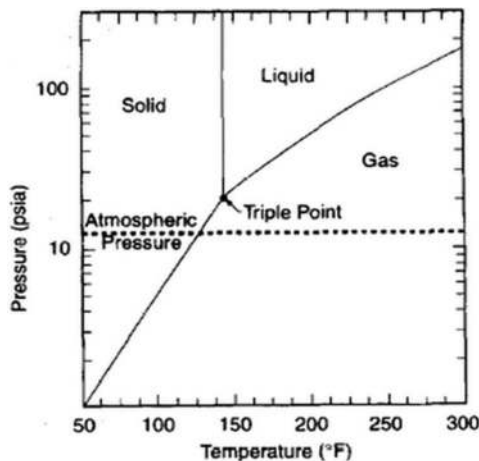
Figure 2. UF_6 phase diagram, showing relationship between pressure, temperature, and physical form [13].
