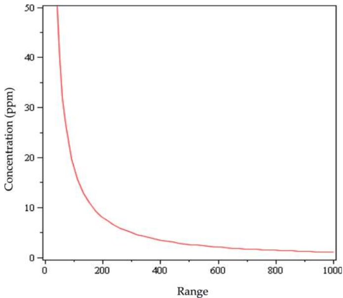
Figure 5. The minimum detectable \text{UF}_6 concentration by DIAL ( \lambda_{\text{on}} = 245 nm and \lambda_{\text{off}} = 266 nm) versus range for one pulse for a very low dark count detector. The SNR is considered to be 1.5. Other parameters of the lidar system are shown in Table 1 .
