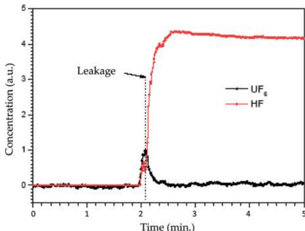
Figure 1. Varying \text{UF}_6 and HF concentration in the moisture atmosphere versus time [11].
