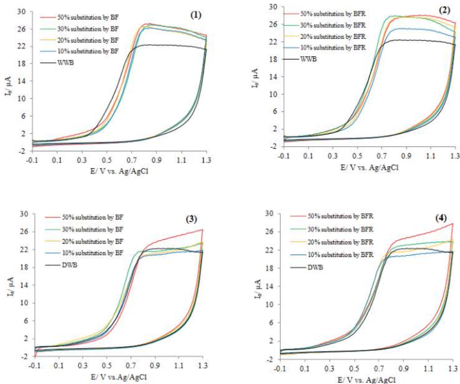
Figure 4. Cyclic voltammograms of soluble fraction obtained after digestion of buckwheat-enhanced white wheat breads (BEWWBs) and buckwheat-enhanced dark wheat breads (BEDWBs). Upper figure, BEWWBs with (1) BF and (2) BFR substitution; lower figure, BEDWBs with (3) BF and (4) BFR substitution. Measurements were performed with soluble fraction obtained after digestion mixed with 0.1 M sodium acetate-acetic buffer (pH 4.5) at ratio 1:1 (v/v) and scan rate 100 \text{ mV s}^{-1} .
