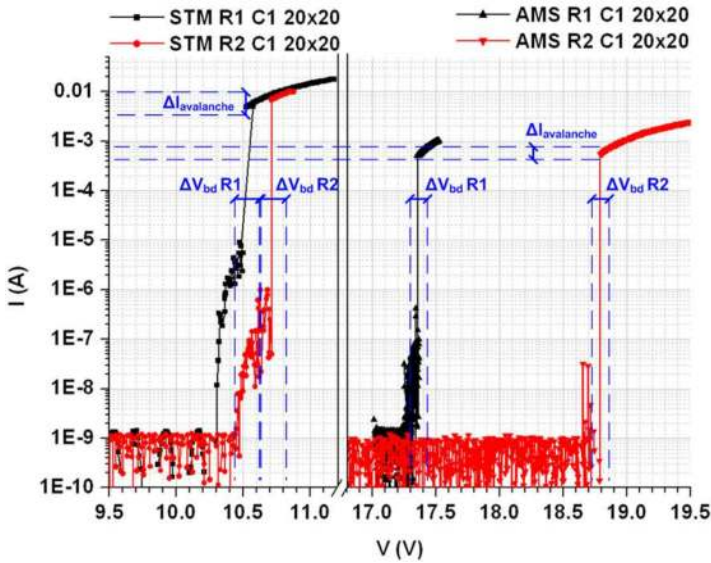
Fig. 7. I-V characteristics of 20µm x 20µm APDs made using STM (left) and HV-AMS (right) technologies, for two different runs (R1 and R2) each.
