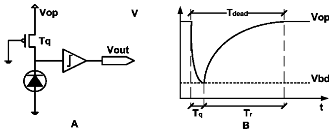
Fig. 15. A) Passive quenching by a transistor and detecting circuits. B) Sketch of the timing behaviour.
