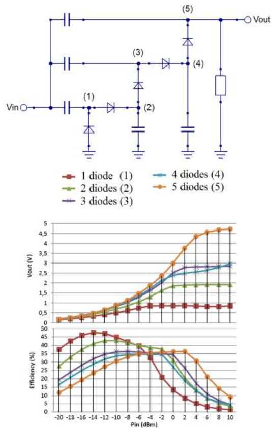
Figure 5. Stages multiplier versus output voltage and efficiency [28].
