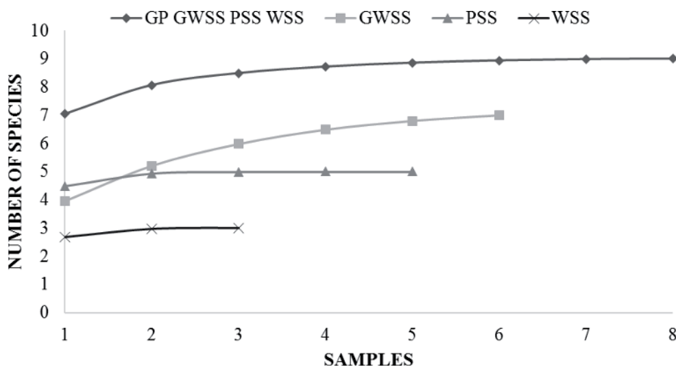
Figure 1. Curve of species accumulation of Tephritinae (Diptera: Tephritidae) in three phytophysiognomies: General Panorama (GP), Grassy-Woody Steppe Savanna (GWS), Park Speppe Savanna (PSS), and Wood Speppe Savanna (WSS), in the Brazilian Chaco (Porto Murtinho-MS) (May 5, 2017 to April 5, 2018).
