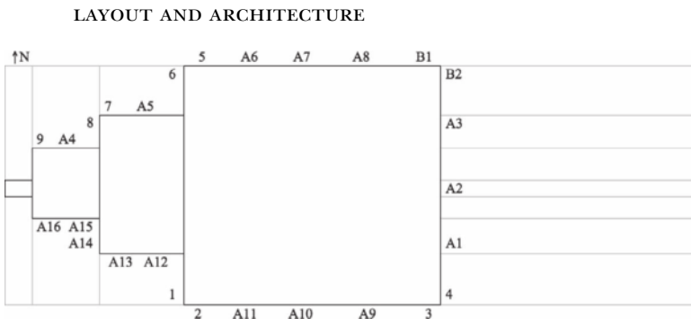
Plate 8.1. Groundplan of Candi Surowono
