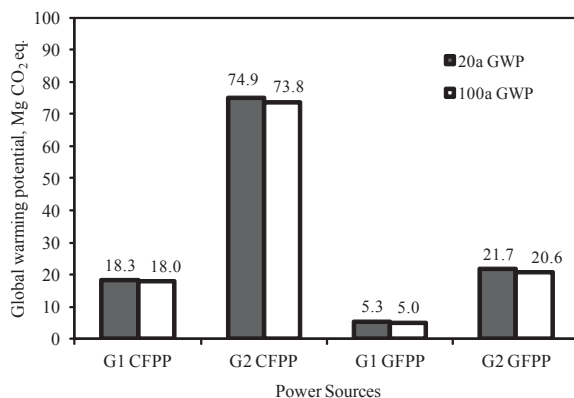
Figure 4. GWP of the GHG emissions derived from the GSHPs heating in G1 and G2.
