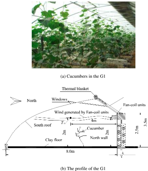
Figure 1. The Chinese solar greenhouse (G1)
