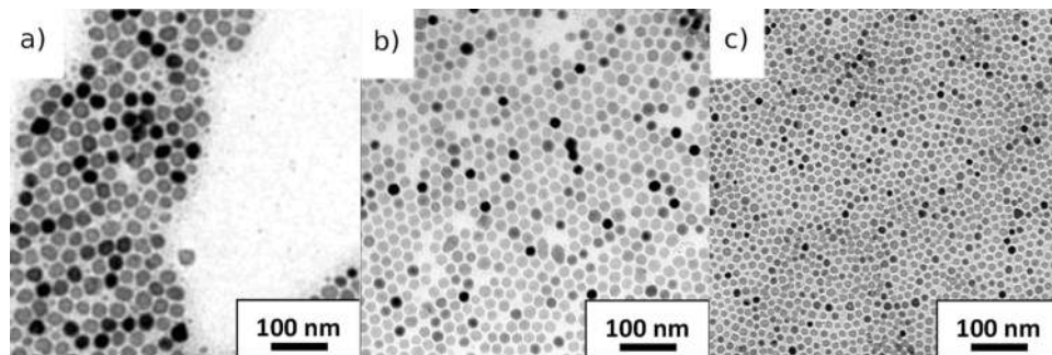
Figure 3. \alpha -MnS NCs by a solvothermal method using sulfur powder in 1-octadecene. (a) 30 nm \alpha -MnS NCs obtained using Mn(OH) 2 as a metal precursor at 300°C. (b) 21 nm \alpha -MnS NCs obtained using Mn(OH) 2 at 320°C. (c) 14 nm \alpha -MnS NCs obtained using Mn(OH)(OH) at 300°C. Adapted from Puglisi A, Mondini S, Cenedese S, Ferretti AM, Santo N, Ponti A. Chem Mater. 2010;22:2804–2813. Ref. [32] Copyright (2010) American Chemical Society.
