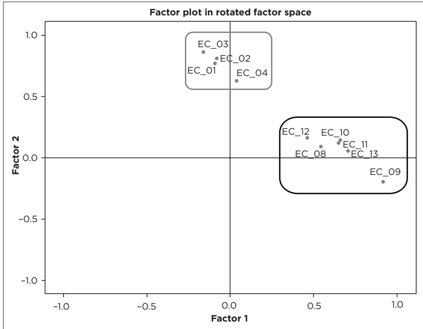
FIGURE 6.8: Environmental complexity factor plot diagram when using Agile.
