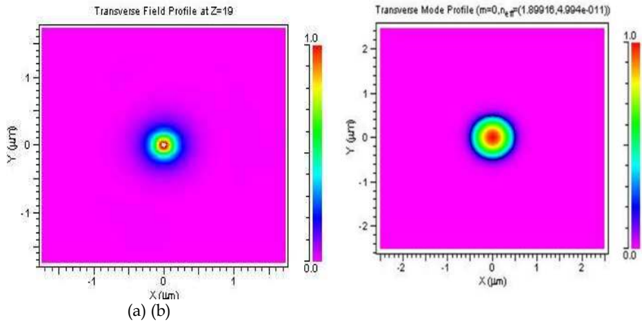
Fig. 12. (a) Transverse field profile prediction for a silicon nitride based CMOS waveguide. The core of the silicon nitride is 0.2 \mu\text{m} in diameter and is embedded in a 1 \mu\text{m} diameter \text{SiO}_2 cladding. (b) Transverse mode field profile for a 0.3 \mu\text{m} oxo-nitride layer embedded in \text{SiO}_2 .
