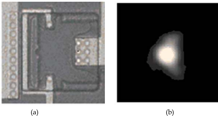
Fig. 7. Si avalanche-based light emitting device (Si Av LED) and electro-optical interfaces realized in 1.2 \mu\text{m} Si CMOS technology with standard CMOS design and processing procedures (Snyman, 1996). (a) Top view with bright field optical microscopy. (b) Optical emission characteristics in dark field conditions
