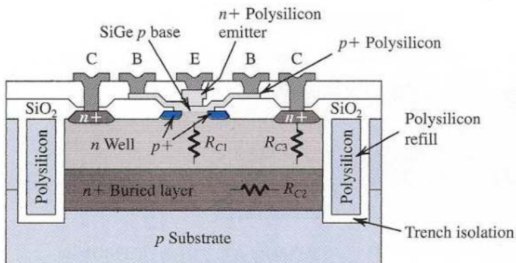
Fig. 4. Components and structural layout of the latest CMOS processes utilising isolation trench based technology (Sedra, 2004).
