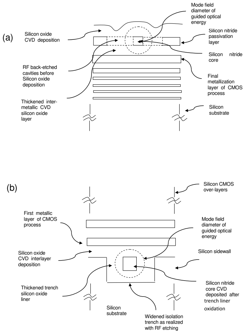
Fig. 5. Cross-sectional profiles of possible wave guides that can be constructed by modification of existing CMOS processes. (a) Waveguide structure fabricated by post processing procedures in the overlayers. (b) Trench based waveguide structure with silicon nitride embedded in silicon oxide.
