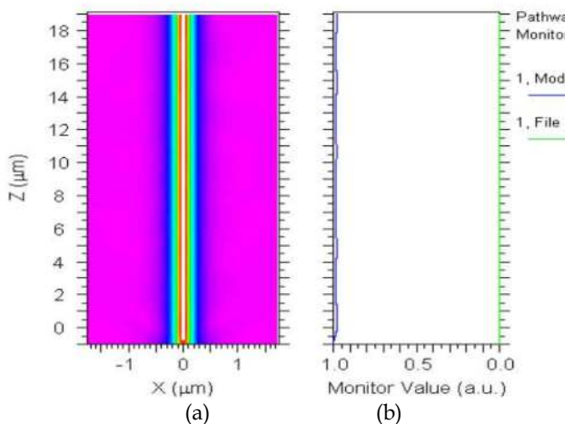
Fig. 11. (a) and (b): Advanced simulation of the electrical field propagation in a silicon nitride layer within CMOS integrated circuitry. Single mode propagation is demonstrated at 750 \text{ nm} over a distance of 20 \mu\text{m} for a 0.2 \mu\text{m} wide silicon nitride waveguide, embedded in \text{SiO}_2 .
