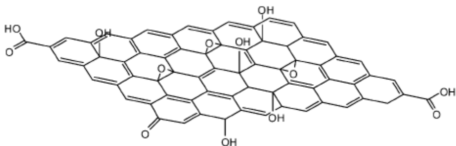
Scheme 5. Graphite oxide (P. Steurer, 2009)
