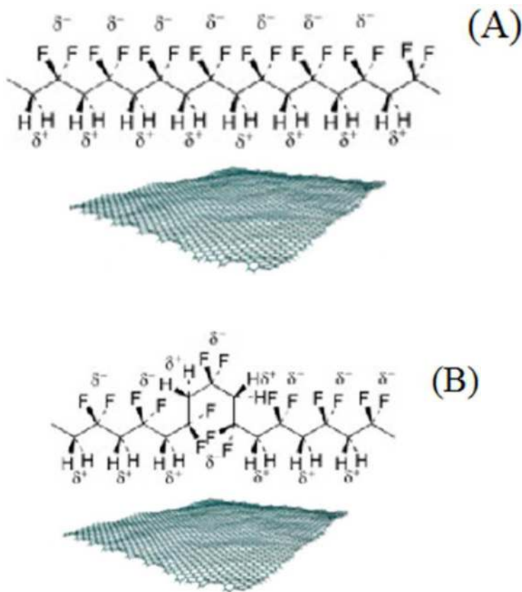
Scheme 7. Schematic illustration of to restricting effect of graphene sheets on TT (A) and TTTG+TTTG- (B) conformation chains
