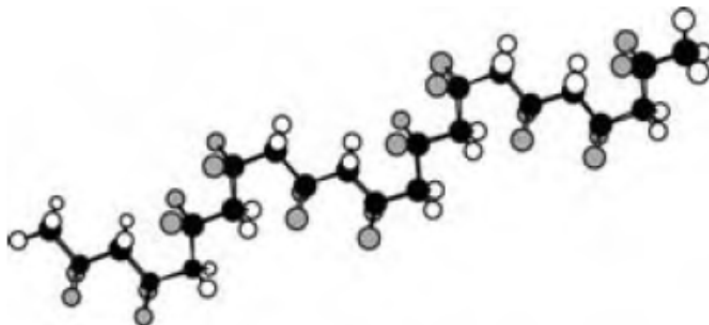
Scheme 4. \gamma and \epsilon crystalline form with T_3G^+T_3G^- conformation (J. H. Yen, 2006)
