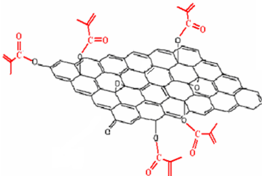
Scheme 6. Modified graphene with methacrylic anhydride (S. Mohamadi, 2011)
