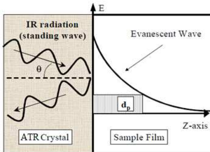
Scheme 1. Schematic illustration of ATR-FTIR configuration (KS. Kwan, 1998)
