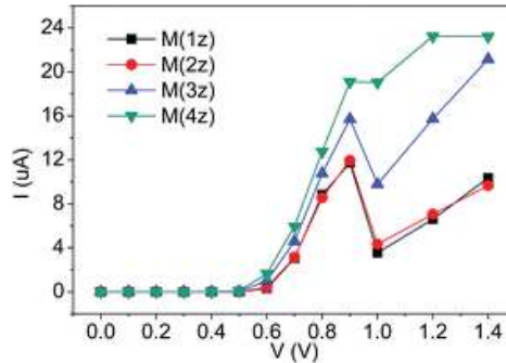
Figure 12. I_d - V_d curves of M(nz) with \text{WS}_2 NR length n ranging from 1 to 4.
