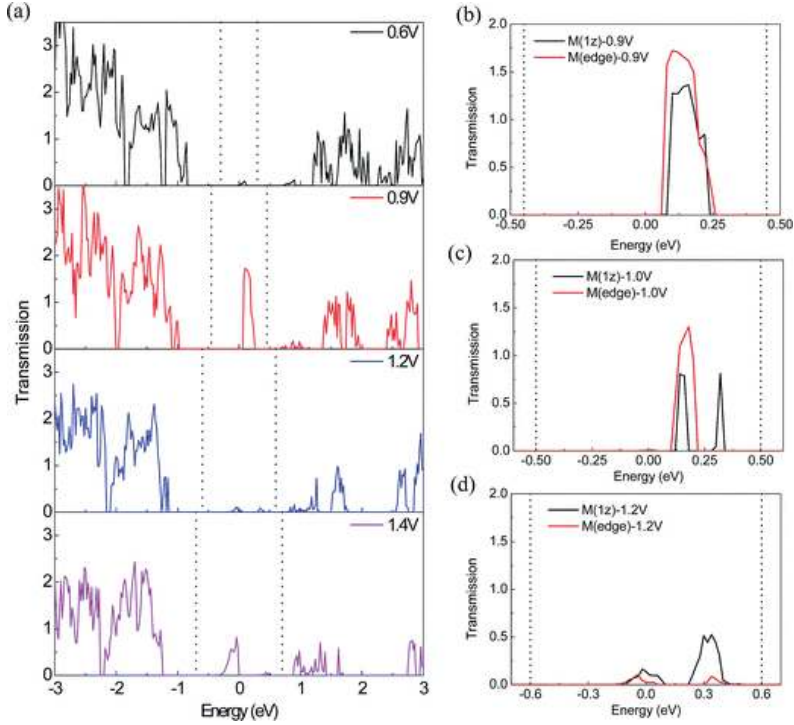
Figure 16. (a) Transmission spectrum for M(edge) at four bias voltages. Dotted line represents the bias window. Transmission spectrum (b) at 0.9 V bias, (c) at 1.0 V bias and (d) at 1.2 V bias for M(1z) and M(edge).
