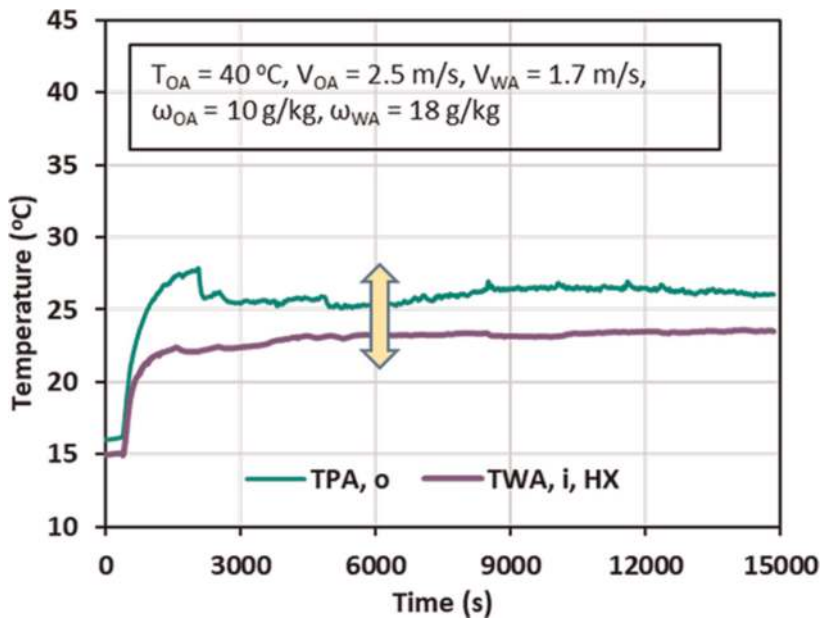
Figure 6. Product air and working air temperature trend.
