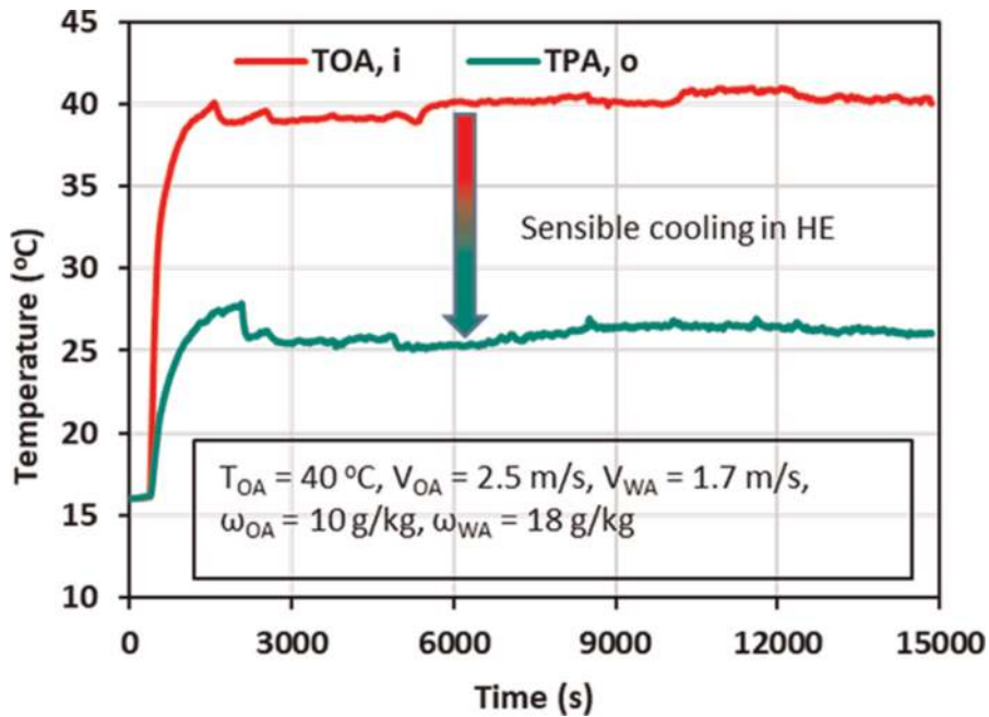
Figure 4. Product air temperature trend.
