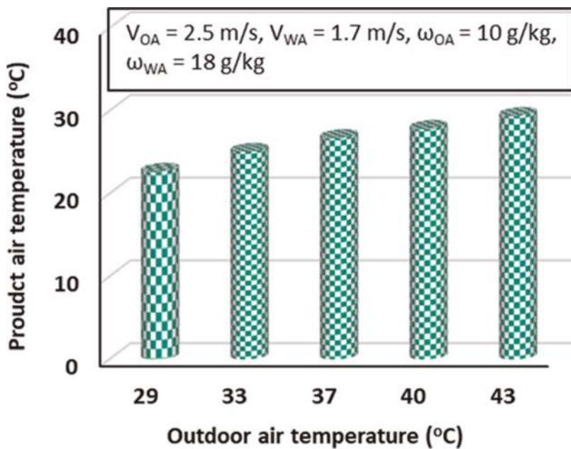
Figure 7. Product air temperature trends at different outer air temperatures.
