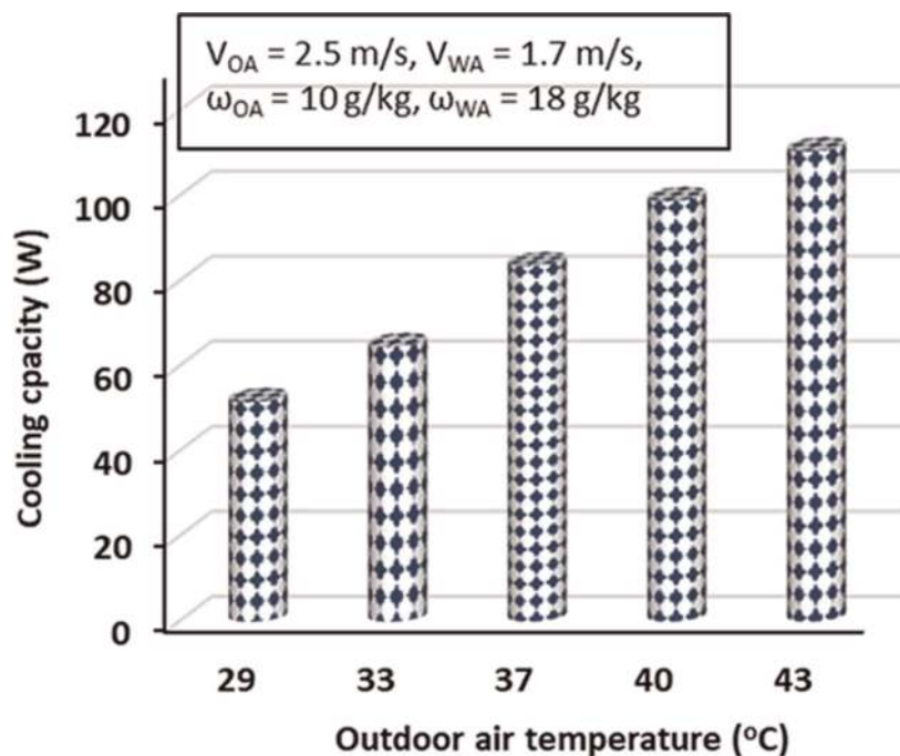
Figure 8. Cooling capacity at different outer air temperatures.
