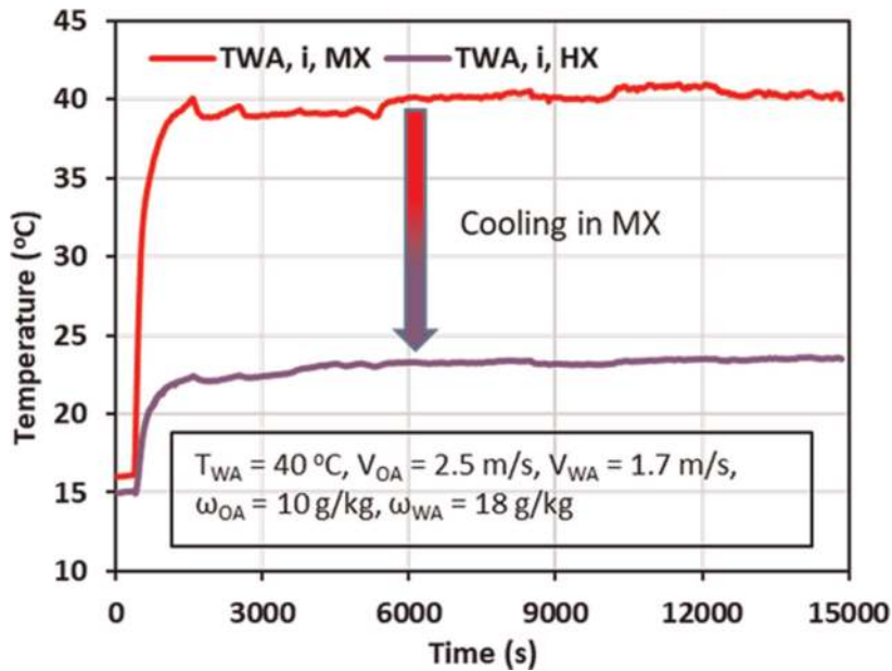
Figure 5. Working air temperature trend.
