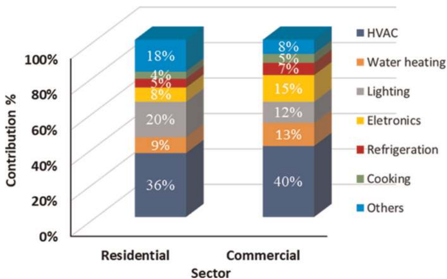
Figure 1. Building energy consumption distribution [8–10].
