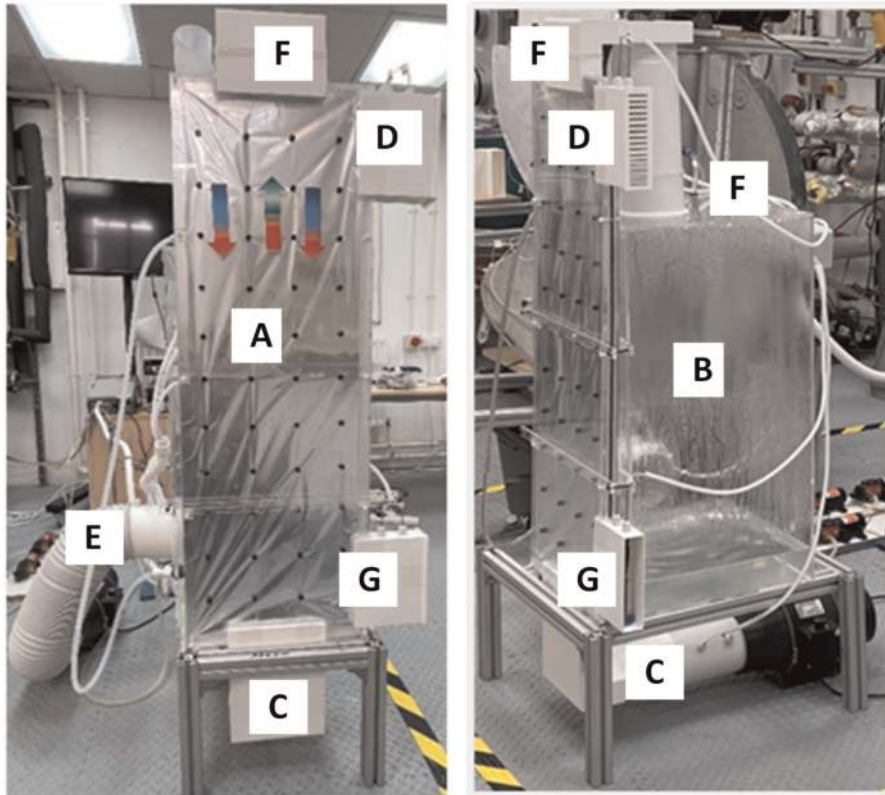
Figure 3. Experimental test rig front and side view.
