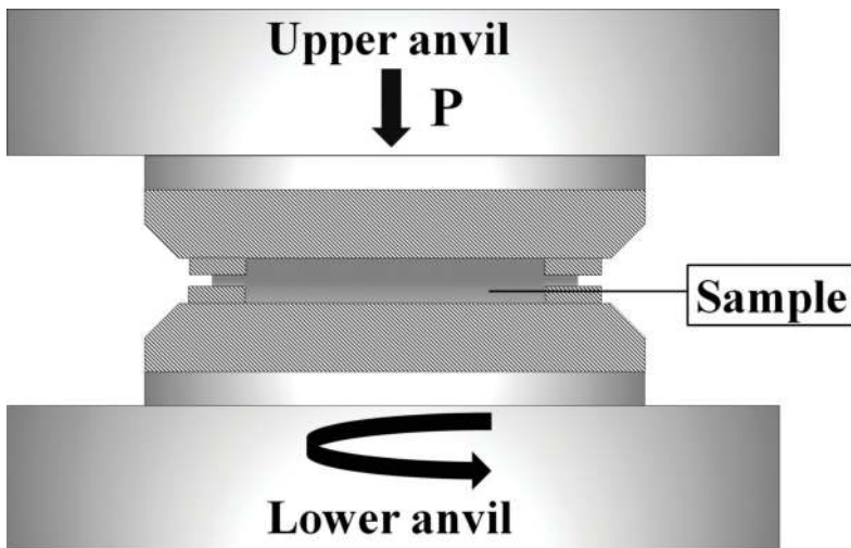
Figure 1. A schematic view of the HPT setup.
