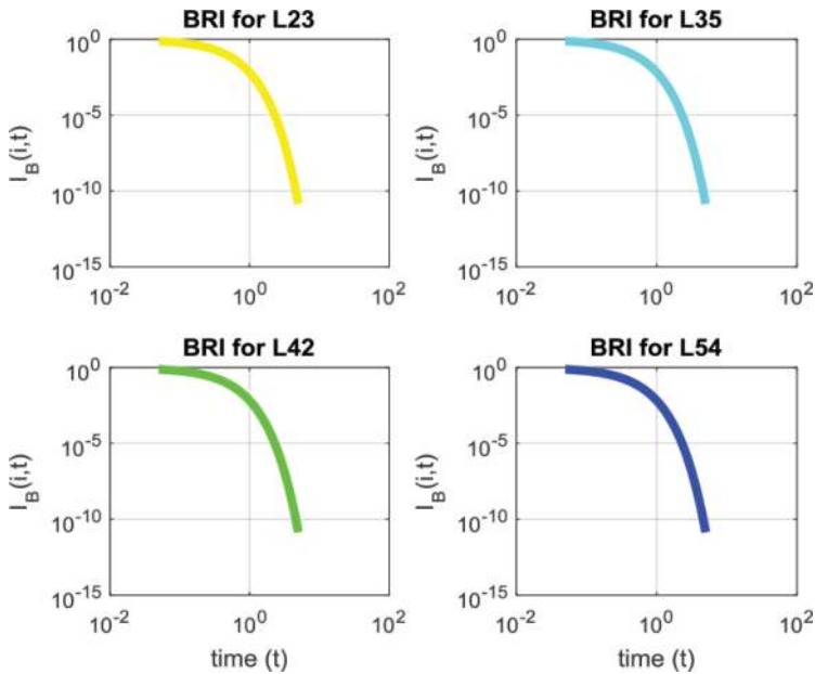
Figure 8. Bimbaum's measure of reliability importance for components: L_{23} , L_{35} , L_{42} , and L_{54} .
