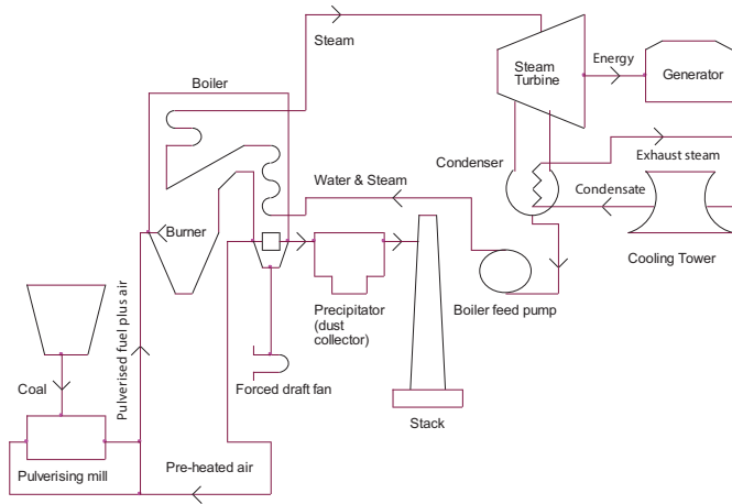
Figure 1. Schematic view of a coal-fired generating station.
