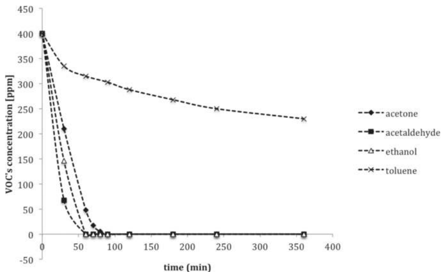
Figure 13. K1077 in the photodegradation of some VOCs.
