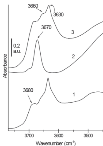
Figure 12. IR. Absorbance IR spectra relative to the OH stretching spectral region of samples outgassed at RT for 60 min: (a) P25; (b) K1077; (c) PC105.
