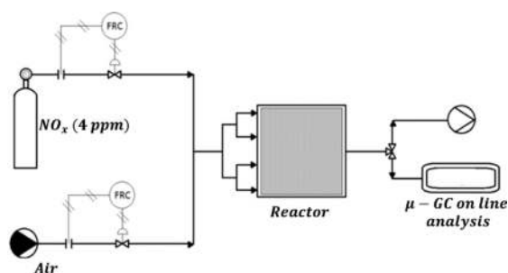
Figure 3. Scheme of the experimental continuous \text{NO}_x set-up.
