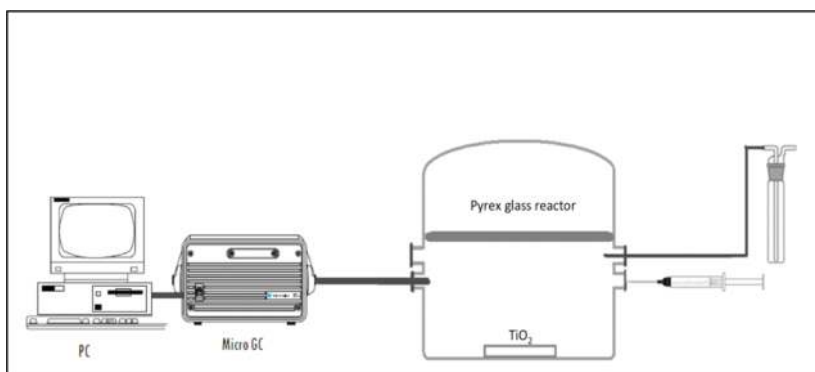
Figure 2. VOC photodegradation—set-up.
