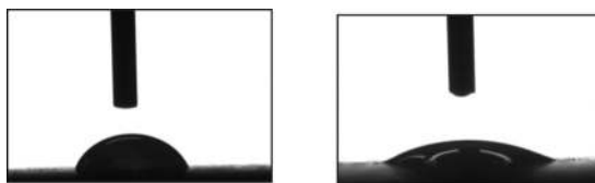
Figure 20. Profile of the water drops at time 0 (image on the left) and at 76 hours (image on the right) on a WGA slab.
