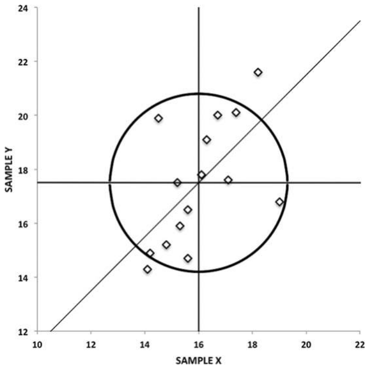
Figure 7. Youden plot (determination of MeP).
