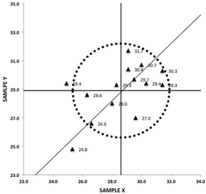
Figure 4. Youden plot (determination of PUFA, BF method).
