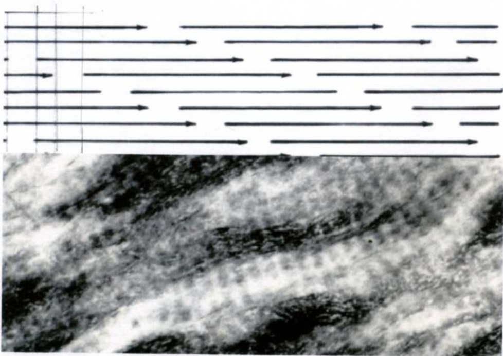
Figure 1. Above: diagram depicting the suggested arrangement of collagen molecules in a fibril: they are shifted in such a way as to generate overlapping (d) and holes (h) zones. Below: in low calcified bone matrix, the inorganic substance is collected in electron-dense bands that cross the collagen fibrils and emphasize their periodic banding. Unstained, x 60,000.
