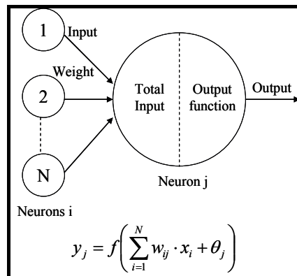
Fig. 1. Generic working of an artificial neuron and its output mathematical representation
