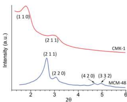
Figure 1. Small-angle XRD patterns of MCM-48 and CMK-1.
