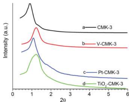
Figure 4. Small-angle XRD patterns of CMK-3 (a), V-CMK-3 (b), Pt-CMK-3 (c), and \text{TiO}_2 -CMK-3 (d).
