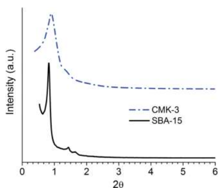
Figure 3. Small-angle XRD patterns of SBA-15 and CMK-3.
