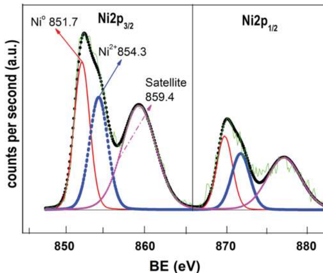
Figure 13. XPS binding energies spectra of the Ni 2p_{3/2} and Ni 2p_{1/2} peaks region separate by a vertical line. Gaussian component: Ni 0 solid line; NiO dot line and satellite peak of NiO dash dot line.
