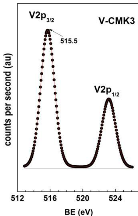
Figure 15. Core level V2p XPS spectra of V-CMK-3.
