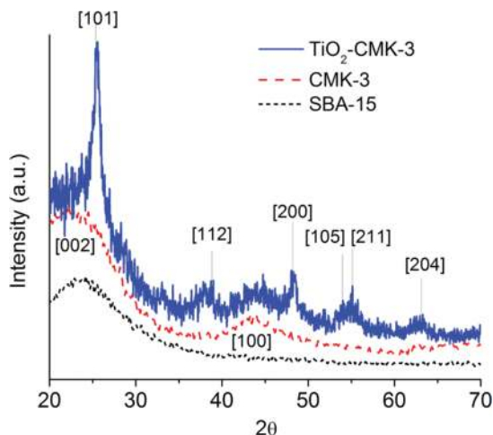
Figure 7. Wide-angle XRD patterns of SBA-15, CMK-3, and \text{TiO}_2 -CMK-3.
