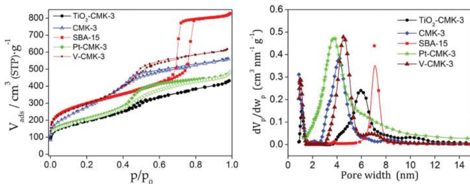
Figure 11. Nitrogen adsorption (solid symbols)–desorption isotherm (open symbols) at 77 K and pore size distribution of (a) SBA-15, (b) CMK-3, (c) Pt-CMK-3, (d) TiO 2 -CMK-3, and (e) V-CMK-3.
