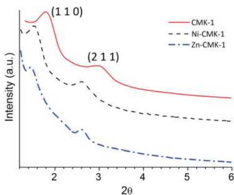
Figure 2. Small-angle XRD patterns of CMK-1, Ni-CMK-1, and Zn-CMK-1.
