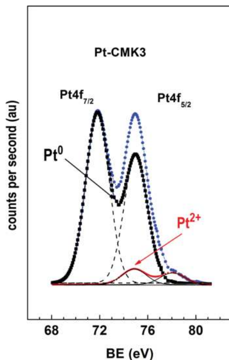
Figure 14. Core level Pt4f XPS spectra of Pt-CMK-3.
