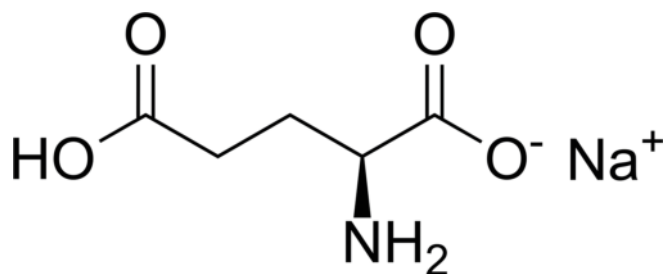
Figure 1. The chemical structure of monosodium glutamate.
