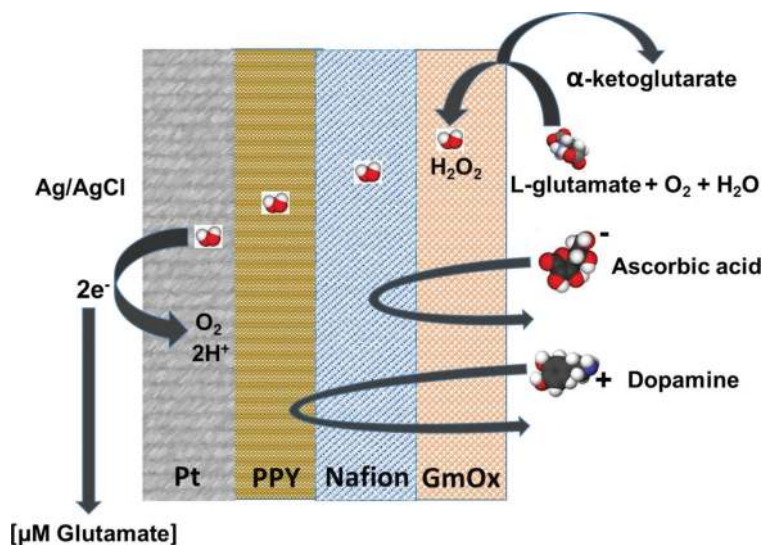
Figure 2. Elimination of interference in glutamate biosensors based on GmOx enzyme.
