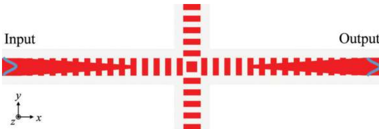
Figure 8. Top view of a SWG-based waveguide crossing.
