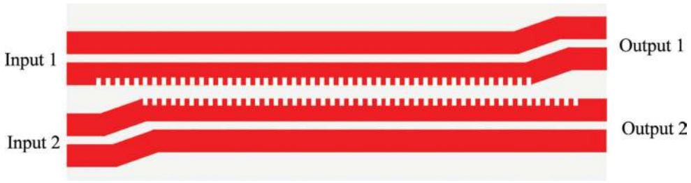
Figure 12. Schematic of a polarization-independent directional coupler based on slot waveguides with SWG structures.
