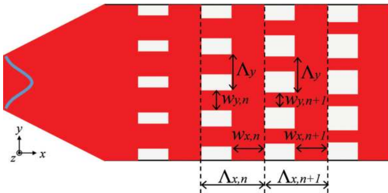
Figure 5. Top view of an apodized grating coupler with crosswise SWG structures.
