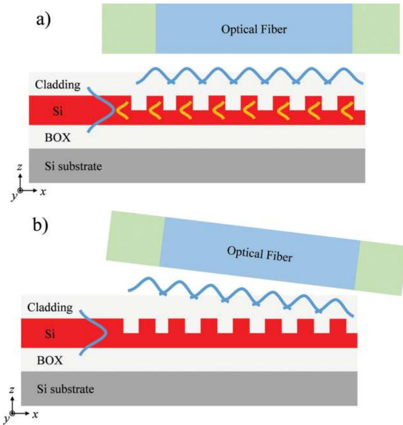
Figure 4. Diagrams describing the concept of a grating coupler working as an output coupler. (a) Vertical first-order diffraction and backward second-order diffraction and (b) tilted first-order diffraction without second-order diffraction.
