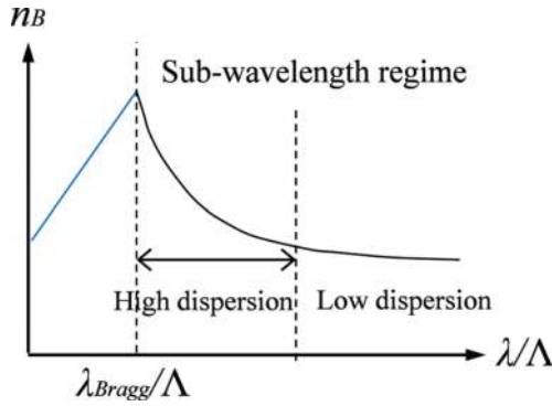
Figure 11. Dispersion in sub-wavelength regime.
