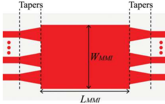
Figure 9. Schematic of a MMI coupler with indications.
