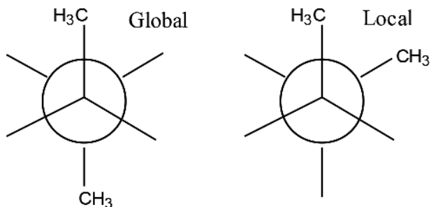
Figure 4. Two different conformations of butane.
