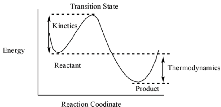
Figure 1. Energy changes during the course of a chemical reaction.
