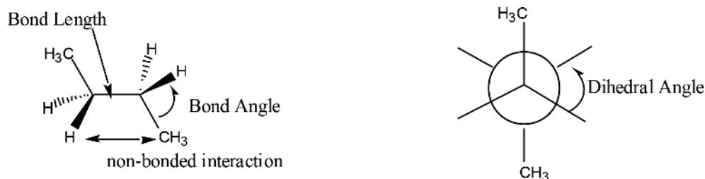
Figure 2. Total energy is affected by bond distances, bond angles, dihedral angles and finally non-bonded interactions.
