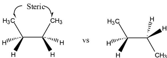
Figure 5. Steric hindrance of a small organic compound.
