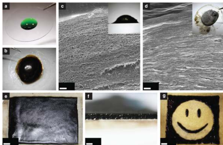
Figure 3. (a) A drop of b-PEI solution was first deposited onto the substrate. (b) When the glass slide was immersed in a GO suspension, a thick film developed over the b-PEI covered area. (c) Foam-like structured 3D graphene paper sample obtained by freeze-drying is revealed by the SEM image. (d) Compact structured graphene paper was prepared by oven drying. (e) A large-area (8 cm × 10 cm) film prepared on a filter paper is photographed. (f and g) This shows the graphene film formed only on the area to which b-PEI was dropped, allowing to pattern the film into a pre-designed shape such as a simplified face shown in (g) [41].
