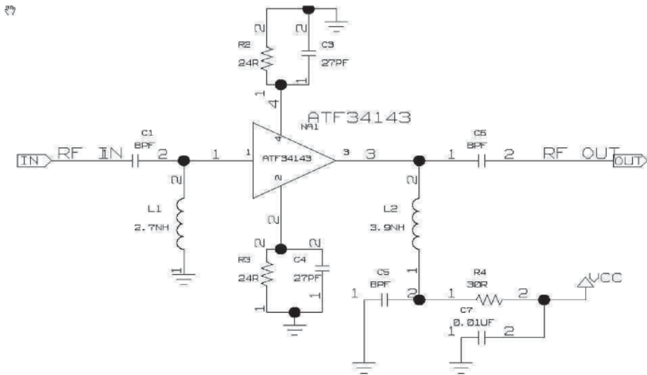
Figure 14. Initial electrical schematic.
