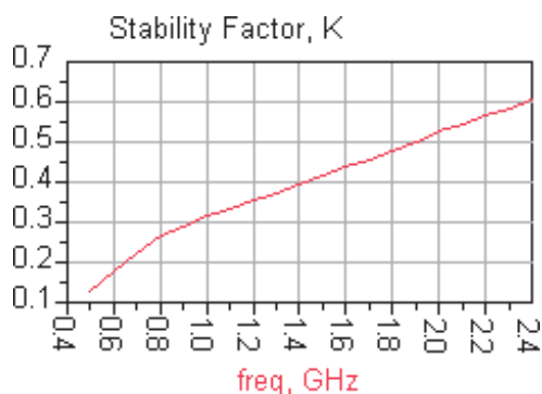
Figure 11. ATF 34143 stability analysis results. (a) Increase the inductance at the source to make the circuit stability greater than 1 in the application frequency range, and then replace the inductance with a microstrip line.
