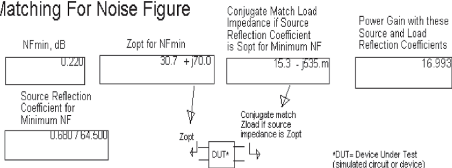
Figure 10. ATF34143 best noise matching conditions.
