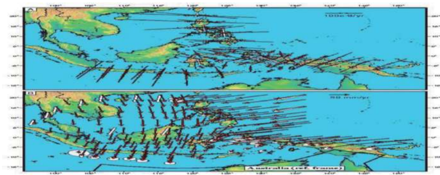
Figure 7. The direction and amount of vectors in the oceanic region of Indian and Pacific plates with relative passiveness of Asian plate.
