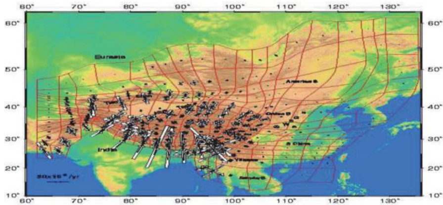
Figure 4. Global Strain Rate Measurement courtesy Zhao.
