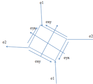
Figure 2. An attempt to explain the nature of strain produced to impending principal (deviatoric) stresses in the horizontal plane over the stratum rock unit: Courtesy: Fundamentals of [19].
