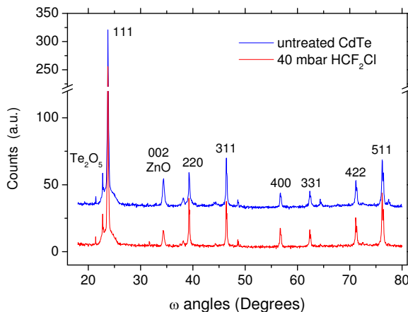
Fig. 4. XRD profiles of the untreated CdTe thin film compared to the sample annealed with 400 mbar Ar+Freon total pressure in the annealing chamber and 40mbar HCF_2Cl partial pressure.
