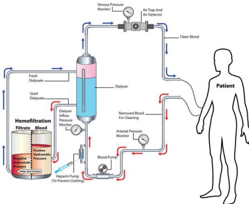
Figure 1. Principle of hemodiafiltration.
