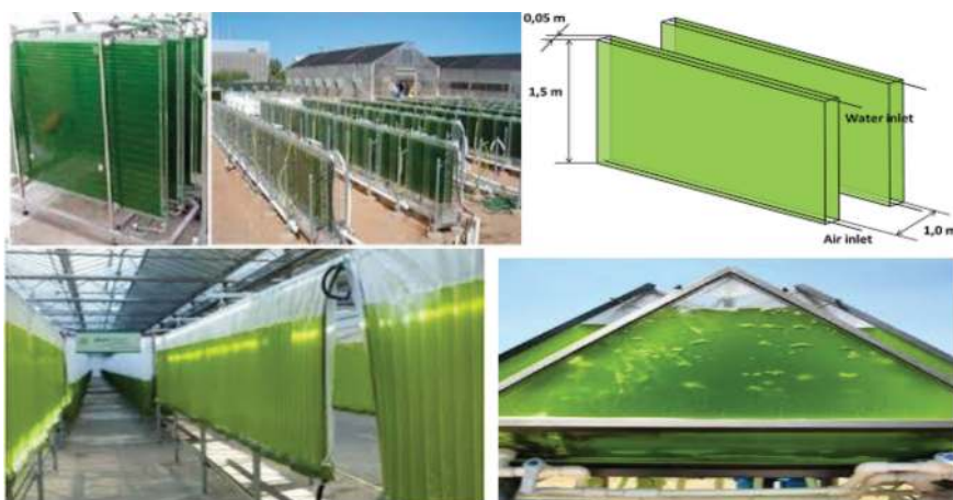
Figure 5. Flat panel photobioreactors.
