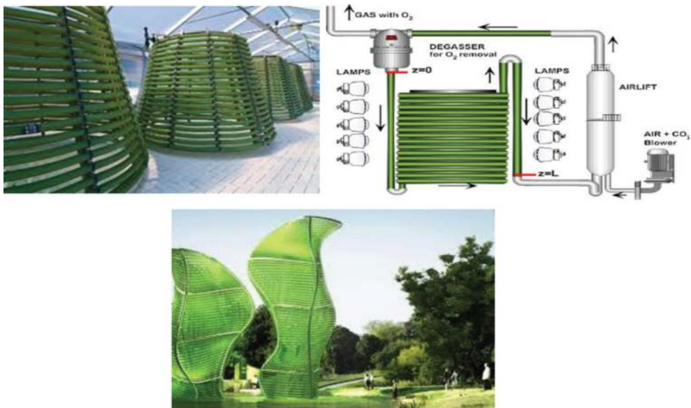
Figure 2. Helical photobioreactor.
