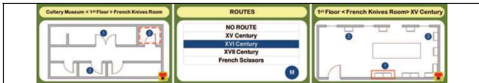
Fig. 9. Routes
