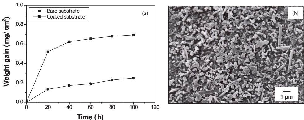
Figure 1. (a) Oxidative weight gain of \text{MgO-Al}_2\text{O}_3\text{-TiO}_2 -based glass-ceramic coated substrate at 1,000^\circ\text{C} for 100 h and (b) typical SEM microstructure of the corresponding coating.
