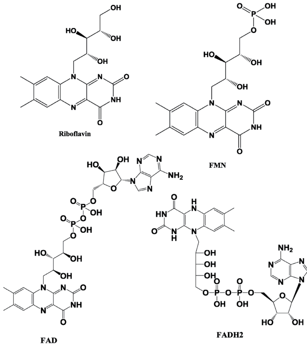
Figure 6. Types of vitamin B2.
