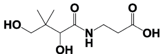
Pantothenic Acid
