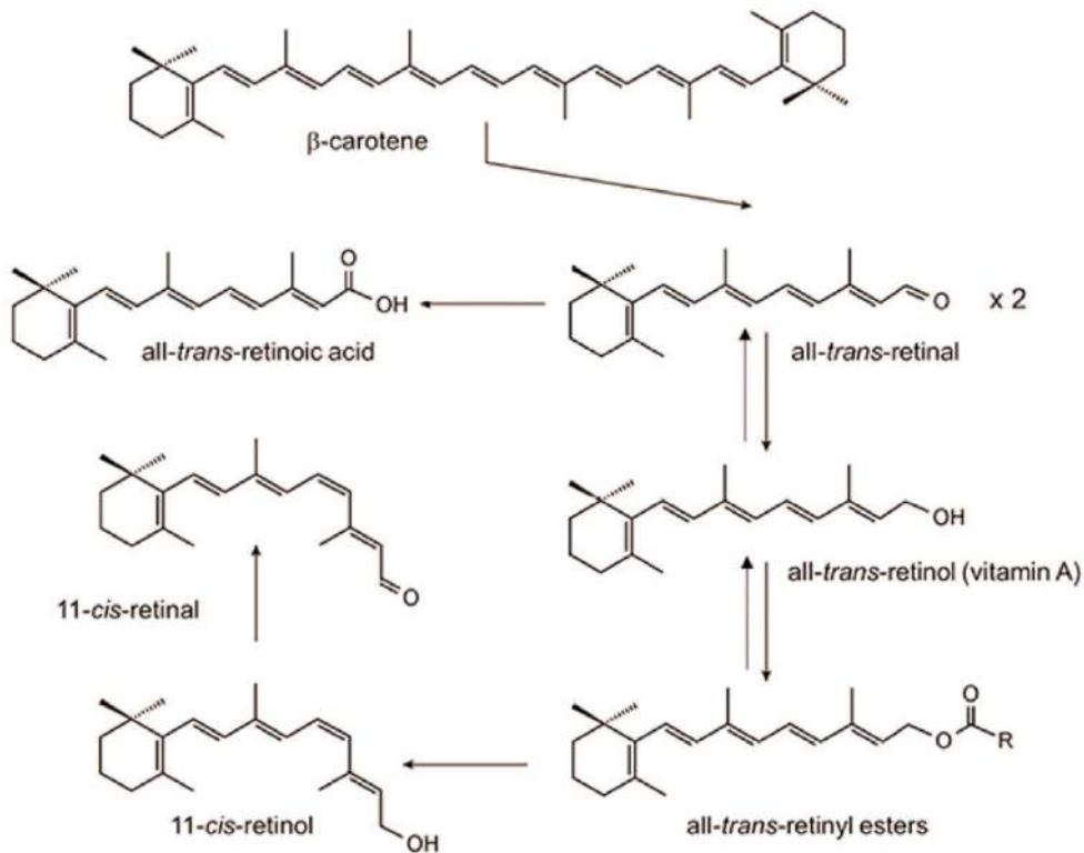
Figure 1. Types of vitamin A.
