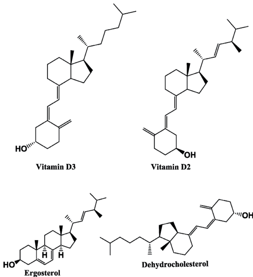
Figure 2. Types of vitamin D.
