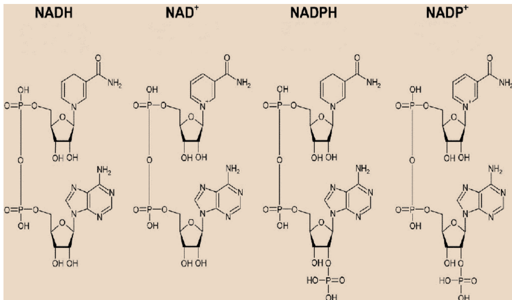
Figure 7. Structures of \text{NADH} , \text{NAD}^+ , \text{NADPH} , and \text{NADP}^+ .
