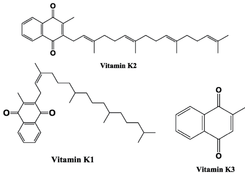
Figure 4. Types of vitamin K.
