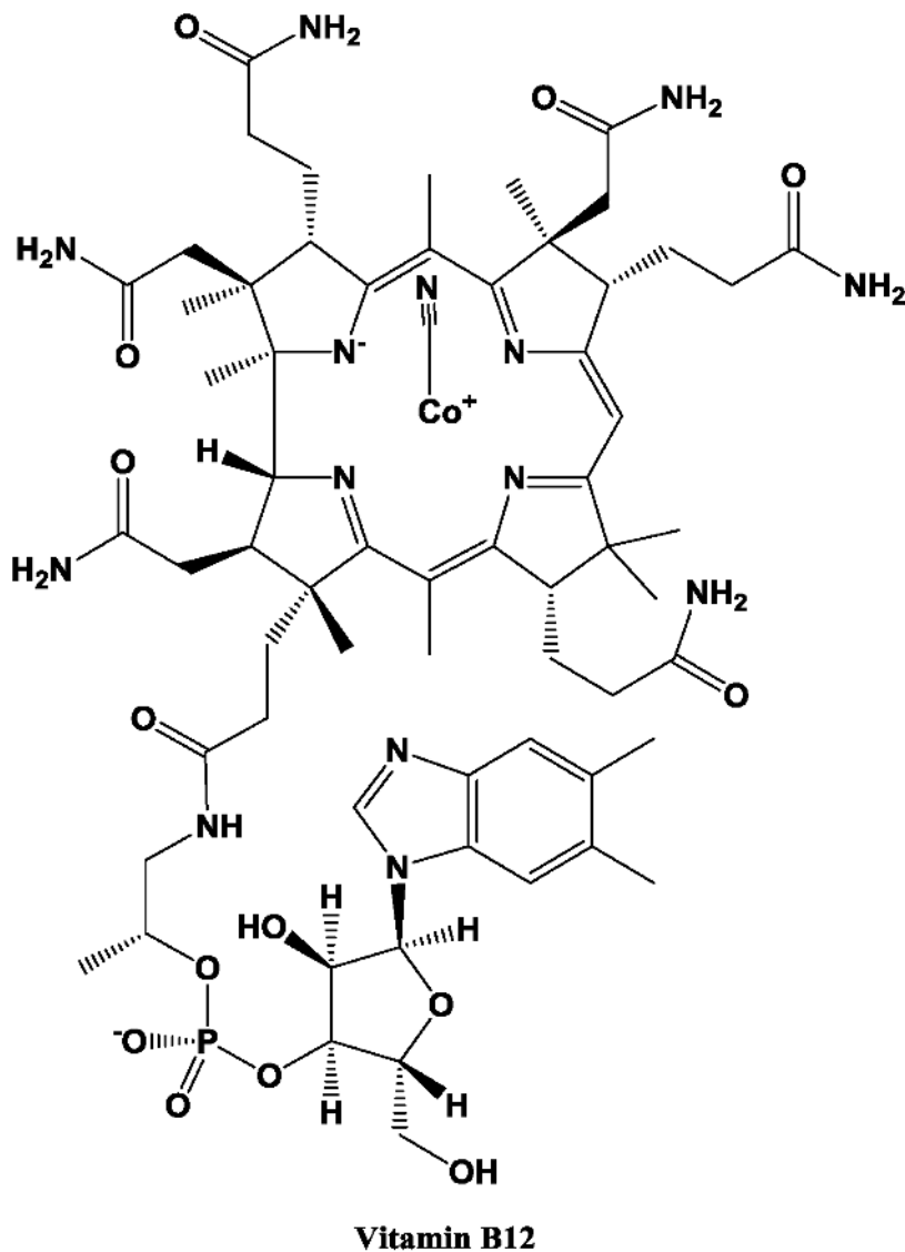
Figure 12. Vitamin B12 (cobalamin).
