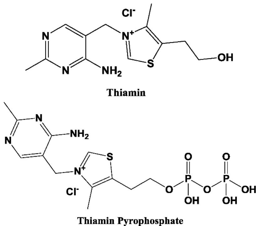
Figure 5. Types of vitamin B1.
