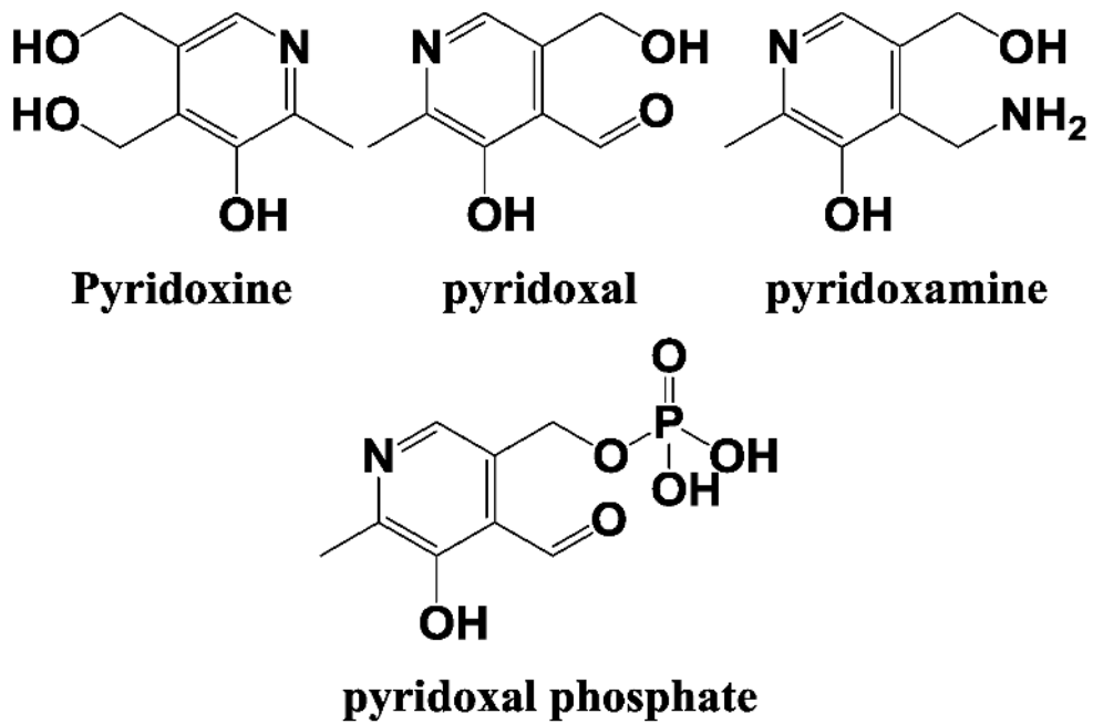
Figure 10. Types of vitamin B6.
