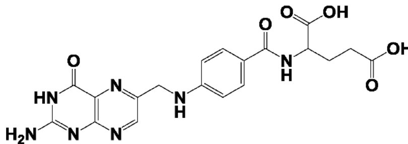
Folic Acid
