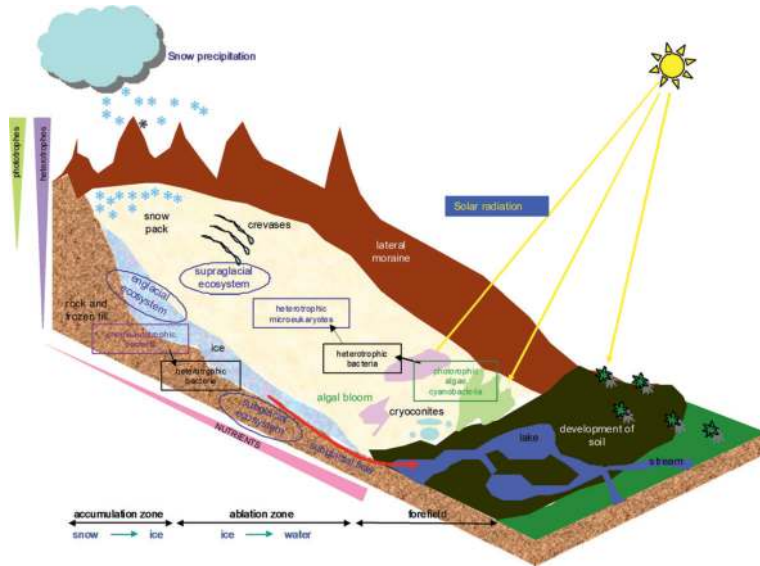
Figure 3. A schematic of different habitats of a glacier colonized by microorganisms. Supraglacial ecosystem is dominated by phototrophic algae and cyanobacteria that take advantage of sunlight and by heterotrophic bacteria and microeukaryotes that feed on organic particles from atmospheric deposition. Microorganisms in englacial ecosystem can be chemoautotrophs, but they can also be heterotrophic bacteria that feed of solubilized products. Subglacial ecosystem is dominated by microorganisms which obtain energy from inorganic compounds and occupy basal ice/till veins and subglacial lakes.
