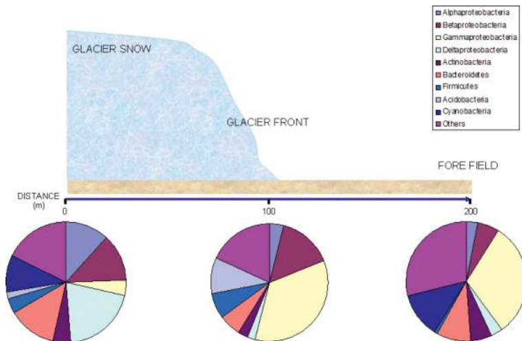
Figure 6. Bacterial community structure along a glacier front based on 16S rRNA gene sequences. Pie charts represent relative abundances of bacterial classes for three glacier environments: glacier snow, glacier front and forefield. The data come from Refs. [51, 76, 77] for glacier snow, from Ref. [6] for glacier front and from Refs. [6, 62, 74] for forefield.
