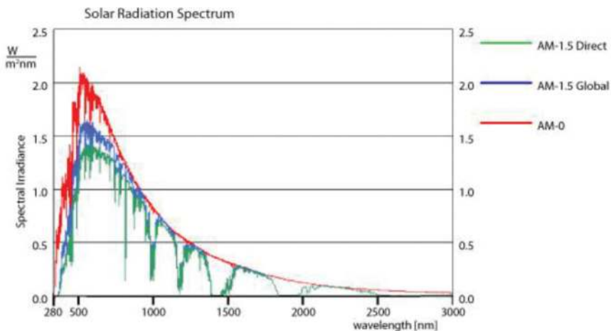
Figure 1. Spectral distribution of radiation intensity [1].
