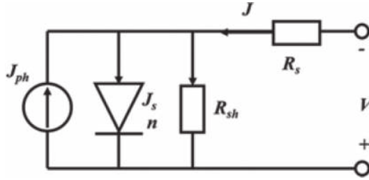
Figure 3. The equivalent circuit of a solar cell.
