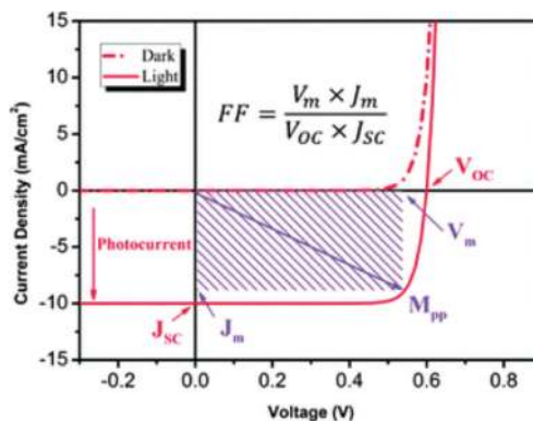
Figure 4. The superposition principle for solar cells.
