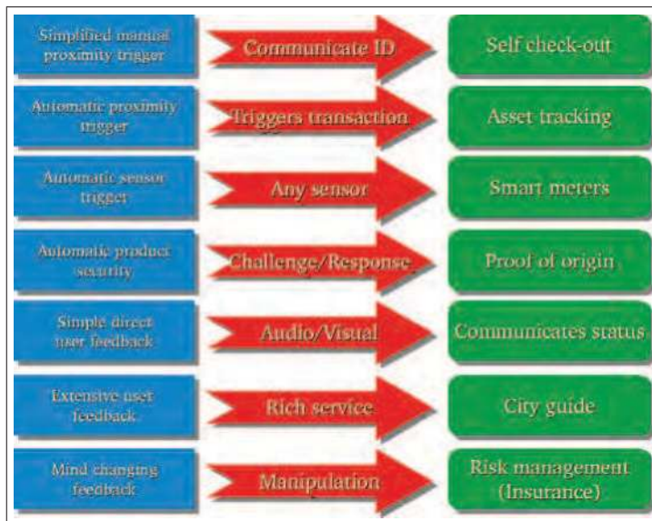
Fig. 6. Internet of Things Application Categorization (Fleisch, 2010)
