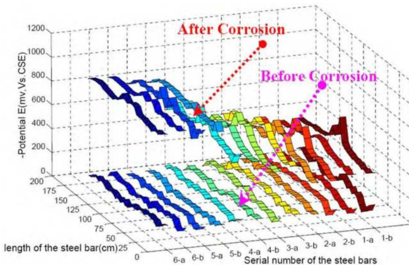
Fig. 25. Half-cell potential of the RC beams
