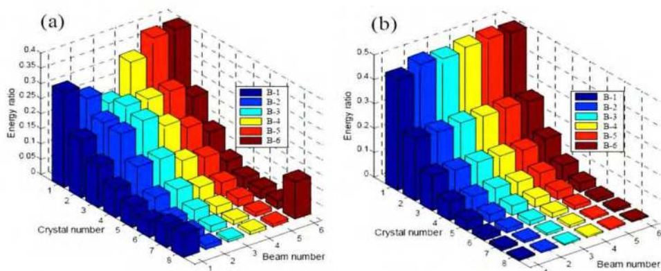
Fig. 29. Energy distribution plot of the EN before corrosion. (a) Electrochemical potential noise. (b) Electrochemical current noise. The histograms whose colors are from dark blue to dark red are the energy distribution plots of the beams which are from the beam1# to the beam 6#. The crystals which are from No.1 to No.8 are the energy concentrated on the different scales. The frequency range of the crystals which are from No.1 to No.8 decrease gradually. So the EN on No.1 level is the most detail part of the EN signal, but the EN on No.8 is much coarser than that of No.1.
