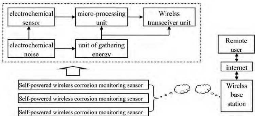
Fig. 22. Self-powered wireless corrosion monitoring networks
