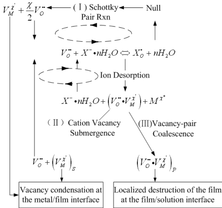
Fig. 3. Postulated reactions for cation vacancy generation at the barrier layer/solution interface according to the Point Defect Model
