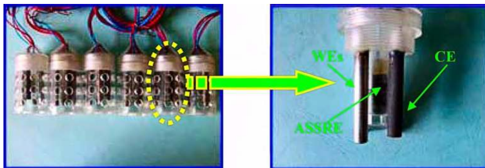
Fig. 20. Five-electrode corrosion sensors
