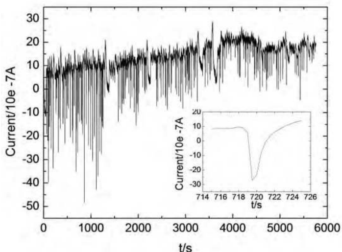
Fig. 14. ECN after 3.0% NaCl solution injected
