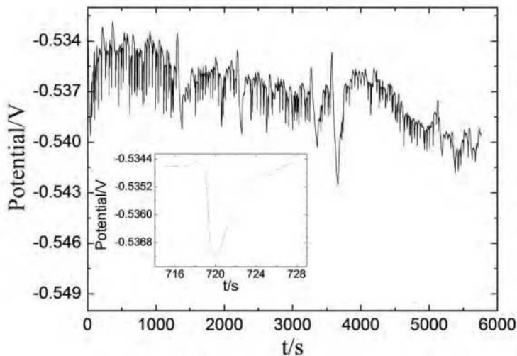
Fig. 13. EPN after 3.0% NaCl solution injected
