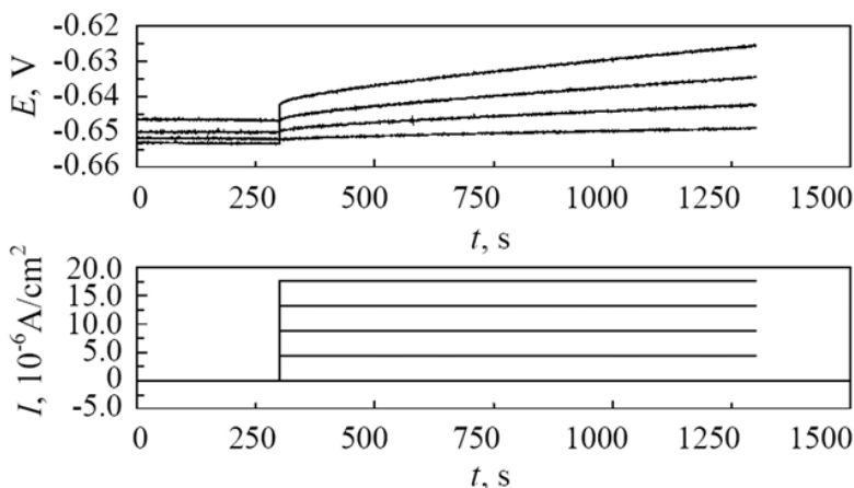
Fig. 26. The potential response of the beam 2#
