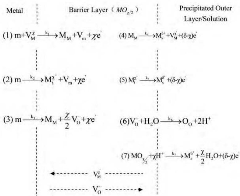
Fig. 2. Schematic of physico-chemical processes that occur within a passive film according to the Point Defect Model
