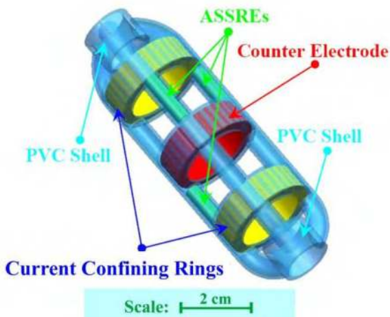
Fig. 21. Solid state and current confining corrosion sensor
