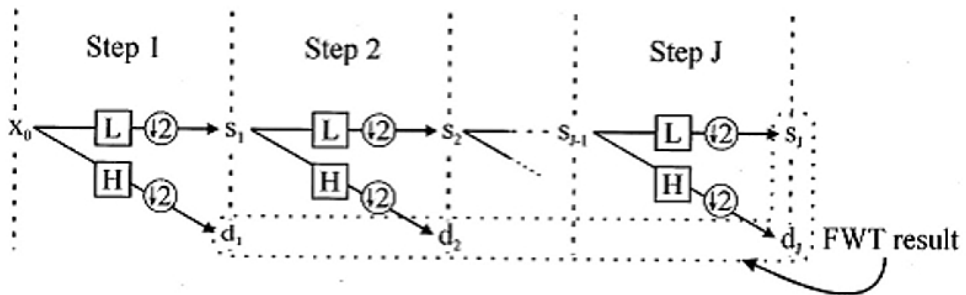
Fig. 10. General scheme of the FWT algorithm
