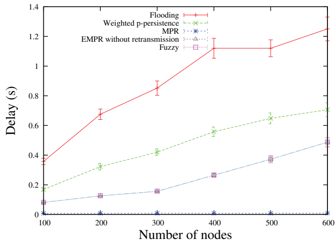
Fig. 13. End-to-end delay for various number of nodes.
