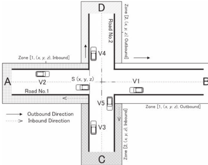
Fig. 3. A street road topology.
