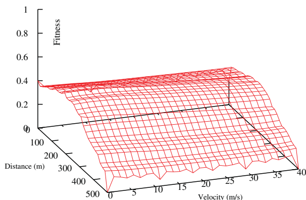
Fig. 12. Relay fitness for various distances and relative velocities.
