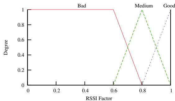
Fig. 6. Signal strength membership function.
