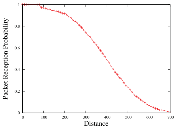
Fig. 9. Packet reception probability for various distances.
