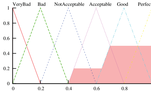
Fig. 8. Output membership function and an example for \mu(x) .
