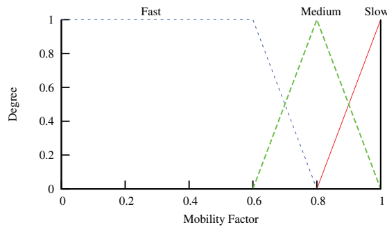
Fig. 5. Mobility membership function.
