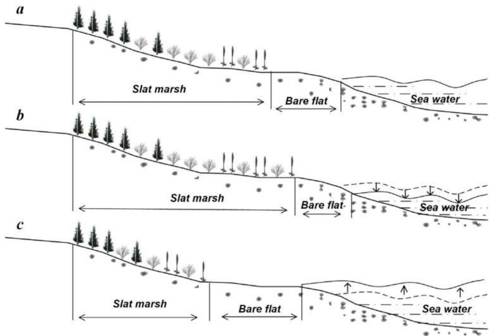
Figure 3. The sketch map of coastal wetland vegetation response to sea level rise. (a) Relative sea level unchanged; (b) relative sea level dropped; (c) relative sea level raised.
