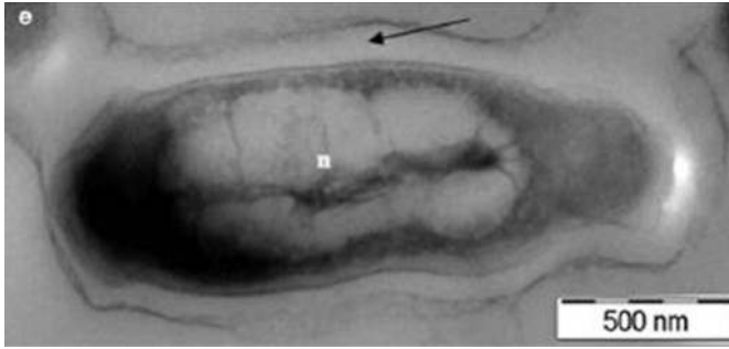
Image 1.1 Transmission electron microscope image of Mycobacterium tuberculosis . The Black arrow indicates the thick mycolic acid layer. The n . indicates the nucleide (from Srinivasan et al., Arch Microbiol, 2014, reprinted with permission)
